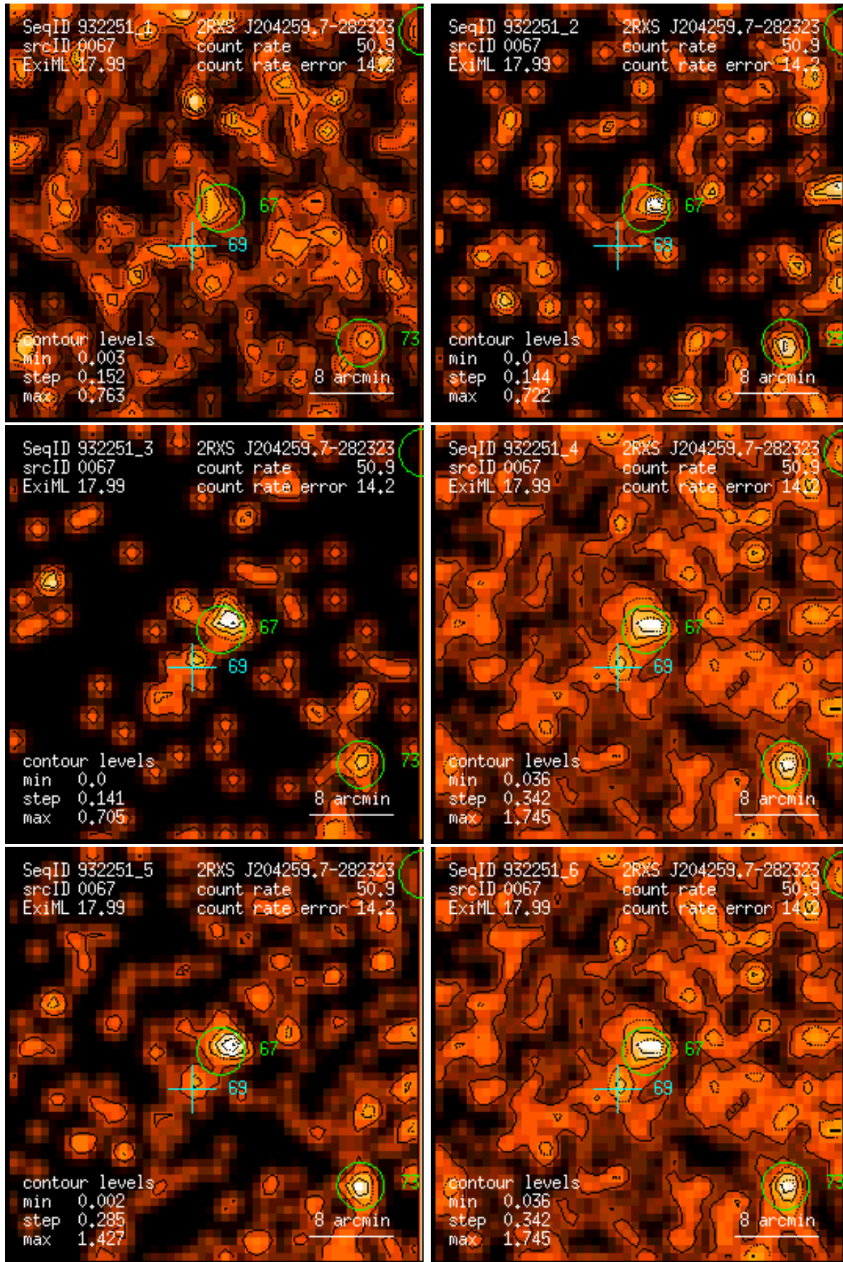
Figure 67: RASS 932251: detection 0067: band rate images, Gaussian filter: (1) PSPC channels 11 – 41, (2) 52 – 90, (3) 91 – 201, (4) 11 – 235, (5) 52 – 201, (6) 11 – 201. Broad band rates in counts/ks. Band rate contour levels in counts/ks/arcmin 2 .
