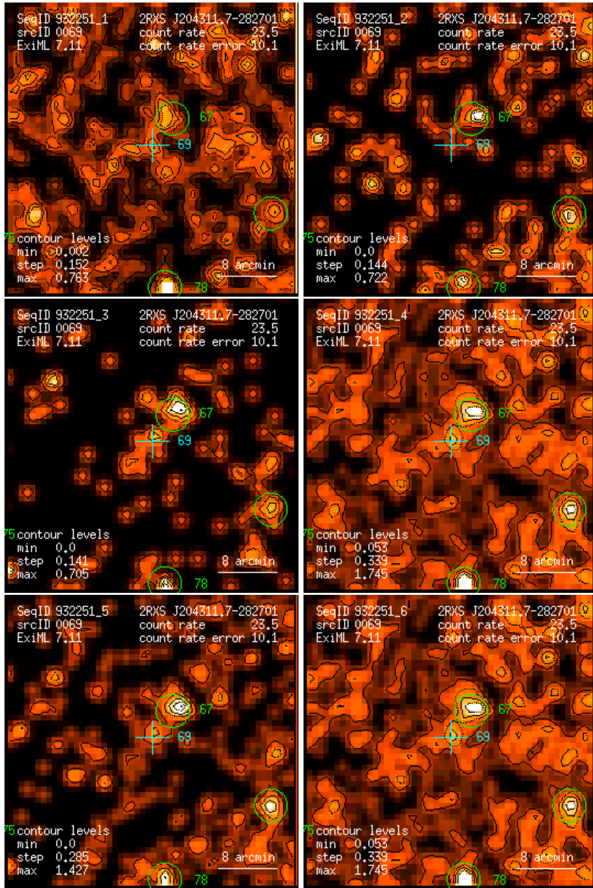
Figure 69: RASS 932251: detection 0069: band rate images, Gaussian filter: (1) PSPC channels 11 – 41, (2) 52 – 90, (3) 91 – 201, (4) 11 – 235, (5) 52 – 201, (6) 11 – 201. Broad band rates in counts/ks. Band rate contour levels in counts/ks/arcmin 2 .
