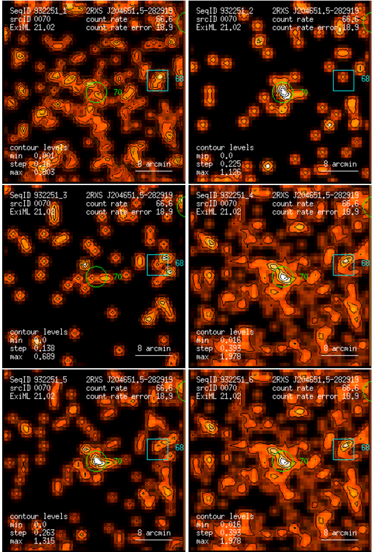
Figure 70: RASS 932251: detection 0070: band rate images, Gaussian filter: (1) PSPC channels 11 – 41, (2) 52 – 90, (3) 91 – 201, (4) 11 – 235, (5) 52 – 201, (6) 11 – 201. Broad band rates in counts/ks. Band rate contour levels in counts/ks/arcmin 2 .
