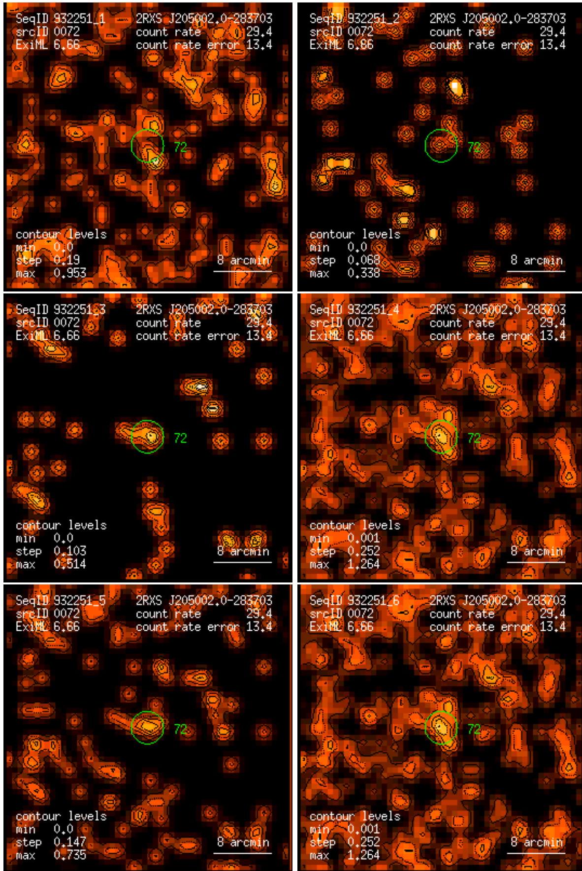
Figure 72: RASS 932251: detection 0072: band rate images, Gaussian filter: (1) PSPC channels 11 – 41, (2) 52 – 90, (3) 91 – 201, (4) 11 – 235, (5) 52 – 201, (6) 11 – 201. Broad band rates in counts/ks. Band rate contour levels in counts/ks/arcmin 2 .
