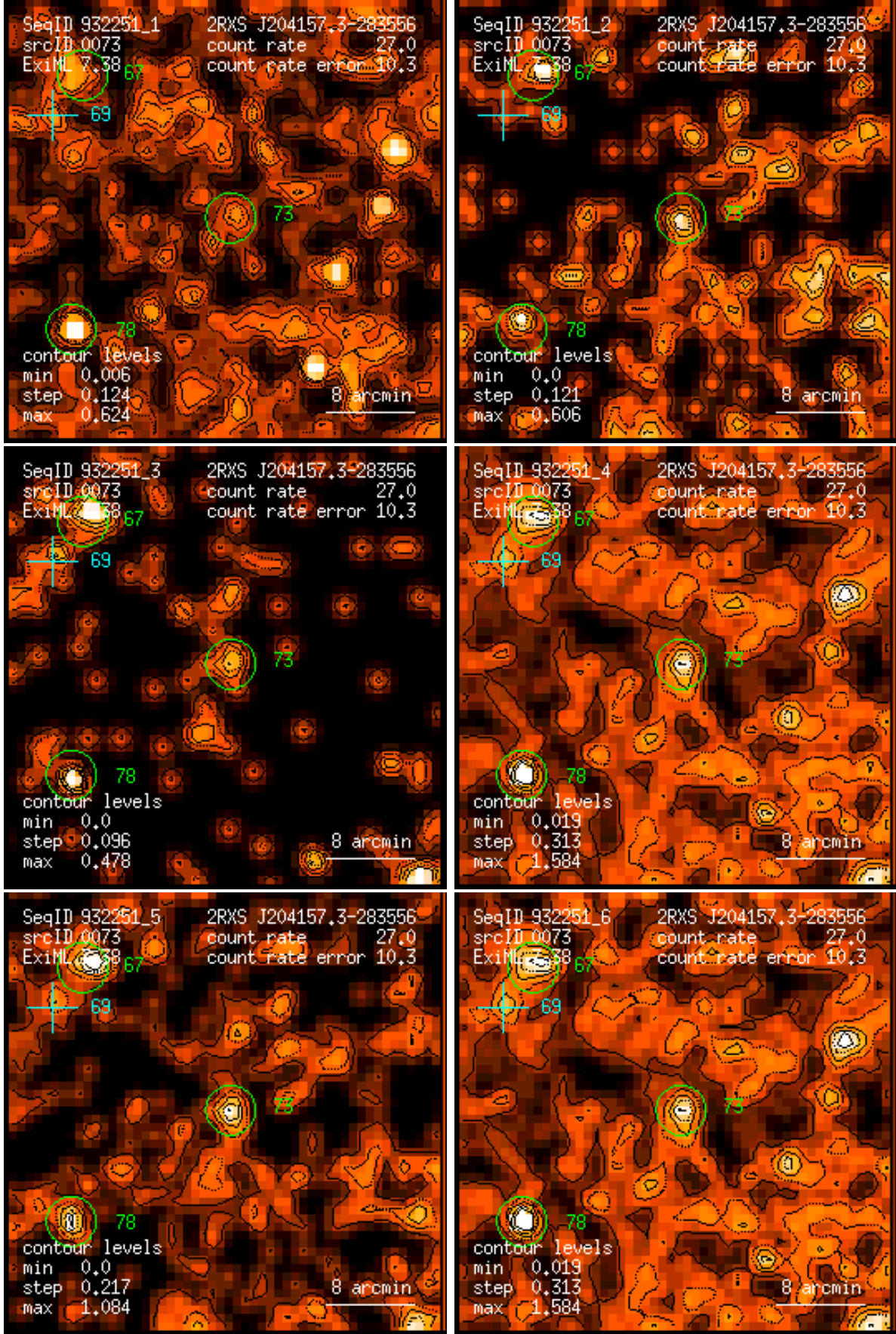
Figure 73: RASS 932251: detection 0073: band rate images, Gaussian filter: (1) PSPC channels 11 – 41, (2) 52 – 90, (3) 91 – 201, (4) 11 – 235, (5) 52 – 201, (6) 11 – 201. Broad band rates in counts/ks. Band rate contour levels in counts/ks/arcmin 2 .
