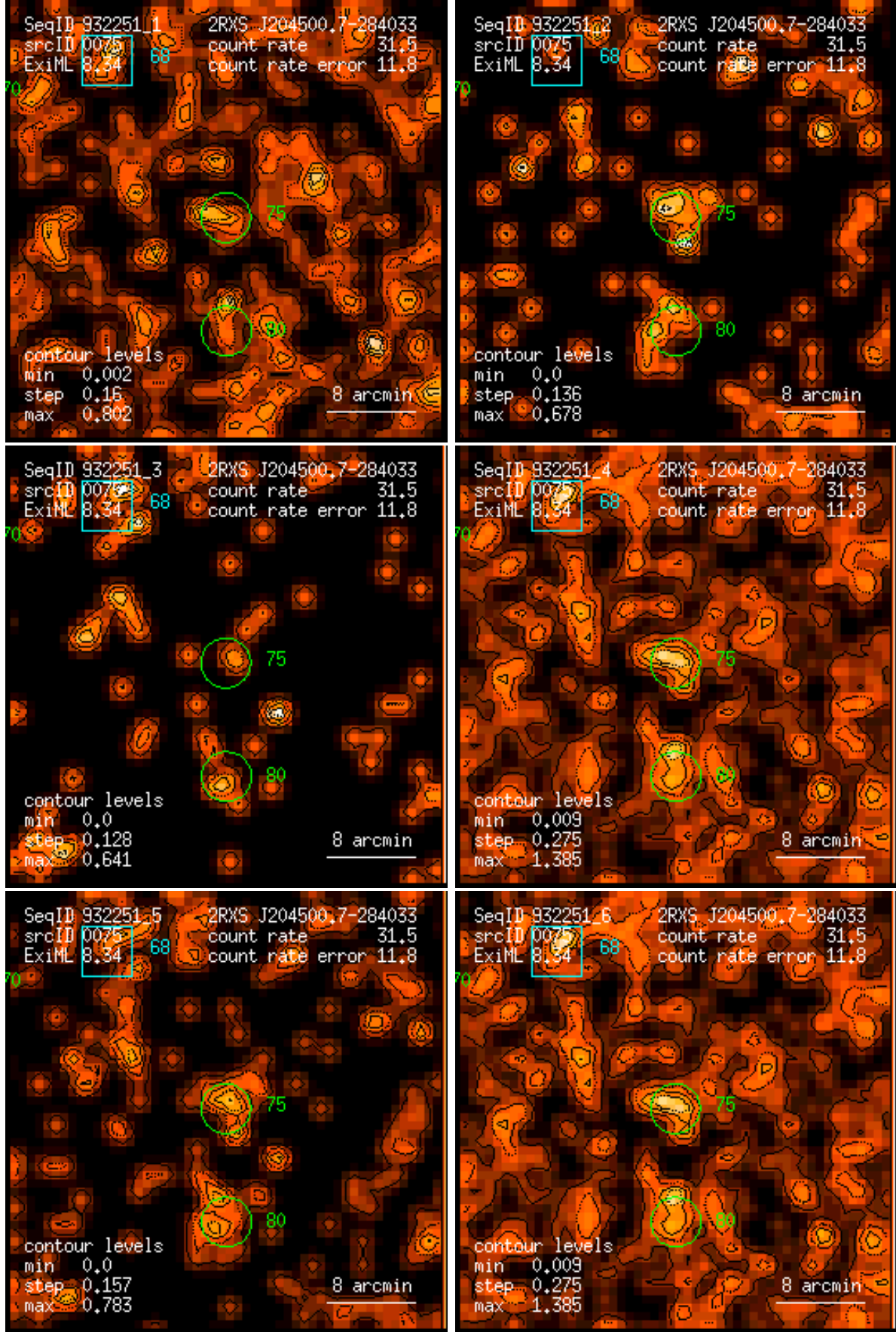
Figure 75: RASS 932251: detection 0075: band rate images, Gaussian filter: (1) PSPC channels 11 – 41, (2) 52 – 90, (3) 91 – 201, (4) 11 – 235, (5) 52 – 201, (6) 11 – 201. Broad band rates in counts/ks. Band rate contour levels in counts/ks/arcmin 2 .
