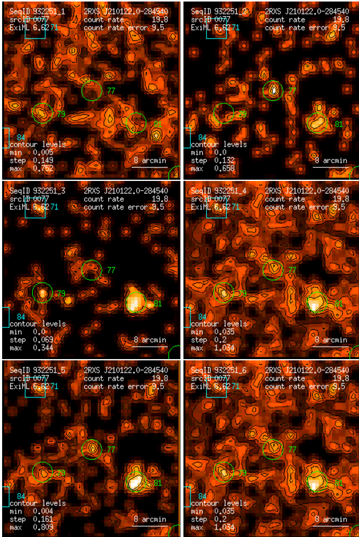
Figure 77: RASS 932251: detection 0077: band rate images, Gaussian filter: (1) PSPC channels 11 – 41, (2) 52 – 90, (3) 91 – 201, (4) 11 – 235, (5) 52 – 201, (6) 11 – 201. Broad band rates in counts/ks. Band rate contour levels in counts/ks/arcmin 2 .
