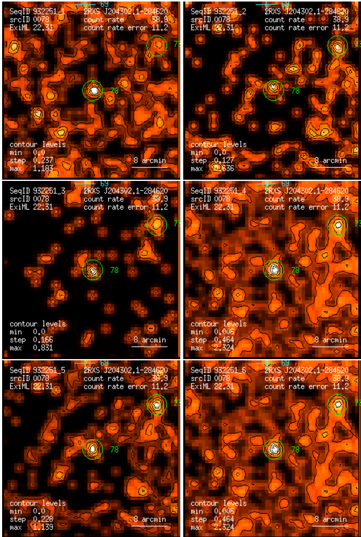
Figure 78: RASS 932251: detection 0078: band rate images, Gaussian filter: (1) PSPC channels 11 – 41, (2) 52 – 90, (3) 91 – 201, (4) 11 – 235, (5) 52 – 201, (6) 11 – 201. Broad band rates in counts/ks. Band rate contour levels in counts/ks/arcmin 2 .
