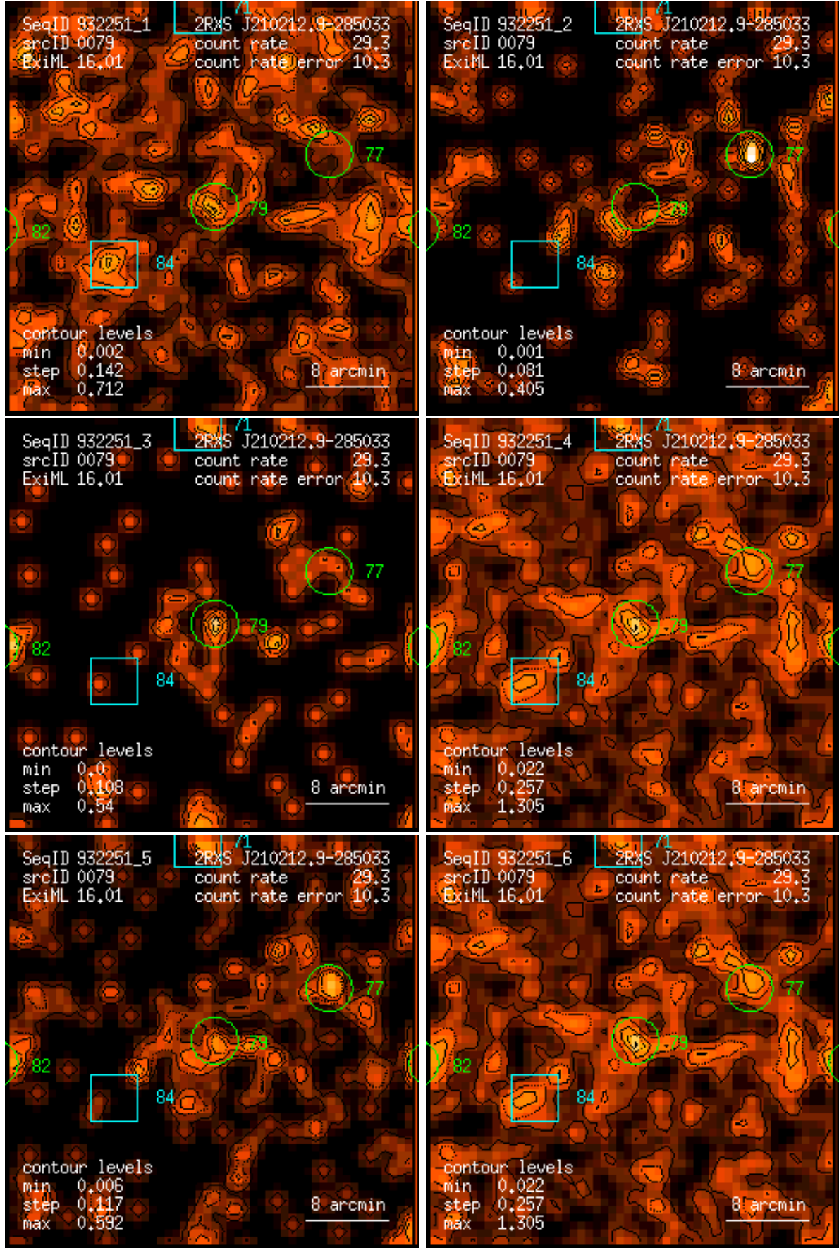
Figure 79: RASS 932251: detection 0079: band rate images, Gaussian filter: (1) PSPC channels 11 – 41, (2) 52 – 90, (3) 91 – 201, (4) 11 – 235, (5) 52 – 201, (6) 11 – 201. Broad band rates in counts/ks. Band rate contour levels in counts/ks/arcmin 2 .
