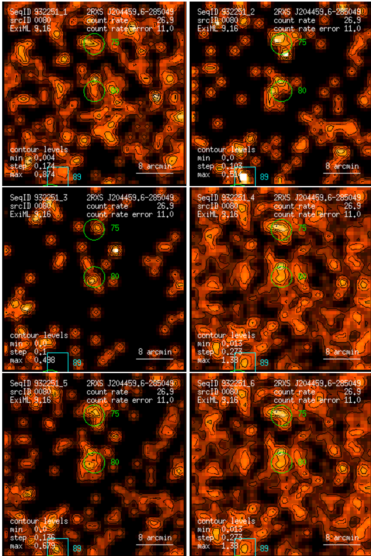
Figure 80: RASS 932251: detection 0080: band rate images, Gaussian filter: (1) PSPC channels 11 – 41, (2) 52 – 90, (3) 91 – 201, (4) 11 – 235, (5) 52 – 201, (6) 11 – 201. Broad band rates in counts/ks. Band rate contour levels in counts/ks/arcmin 2 .
