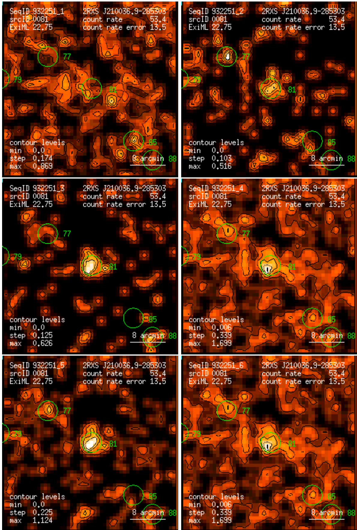
Figure 81: RASS 932251: detection 0081: band rate images, Gaussian filter: (1) PSPC channels 11 – 41, (2) 52 – 90, (3) 91 – 201, (4) 11 – 235, (5) 52 – 201, (6) 11 – 201. Broad band rates in counts/ks. Band rate contour levels in counts/ks/arcmin 2 .
