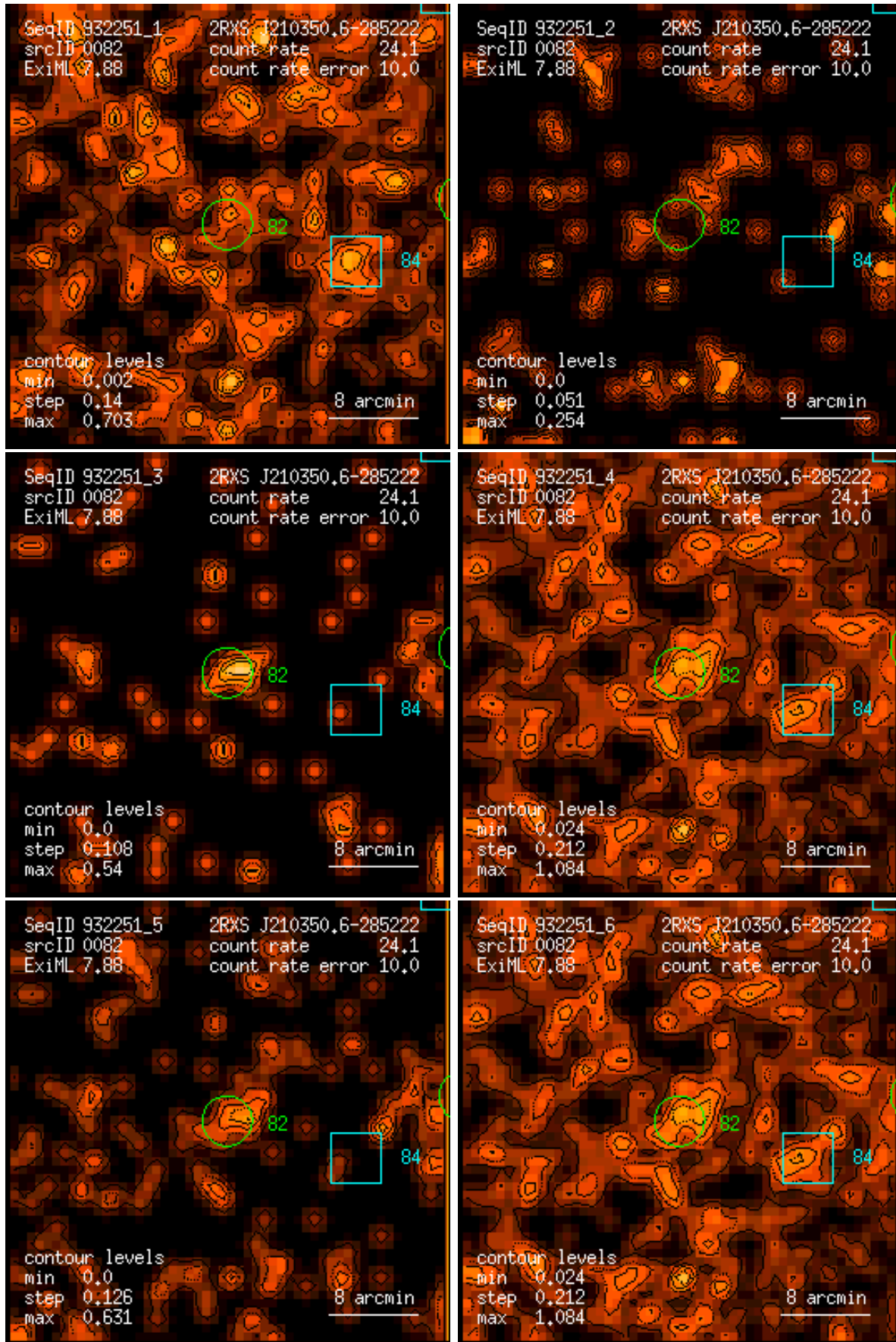
Figure 82: RASS 932251: detection 0082: band rate images, Gaussian filter: (1) PSPC channels 11 – 41, (2) 52 – 90, (3) 91 – 201, (4) 11 – 235, (5) 52 – 201, (6) 11 – 201. Broad band rates in counts/ks. Band rate contour levels in counts/ks/arcmin 2 .
