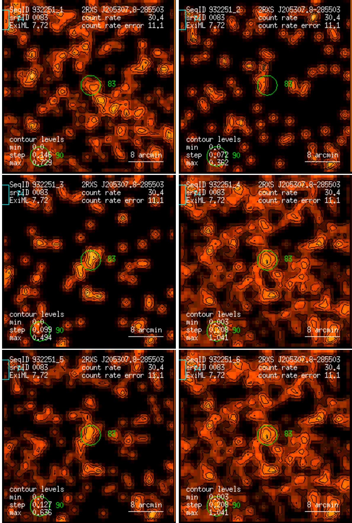
Figure 83: RASS 932251: detection 0083: band rate images, Gaussian filter: (1) PSPC channels 11 – 41, (2) 52 – 90, (3) 91 – 201, (4) 11 – 235, (5) 52 – 201, (6) 11 – 201. Broad band rates in counts/ks. Band rate contour levels in counts/ks/arcmin 2 .
