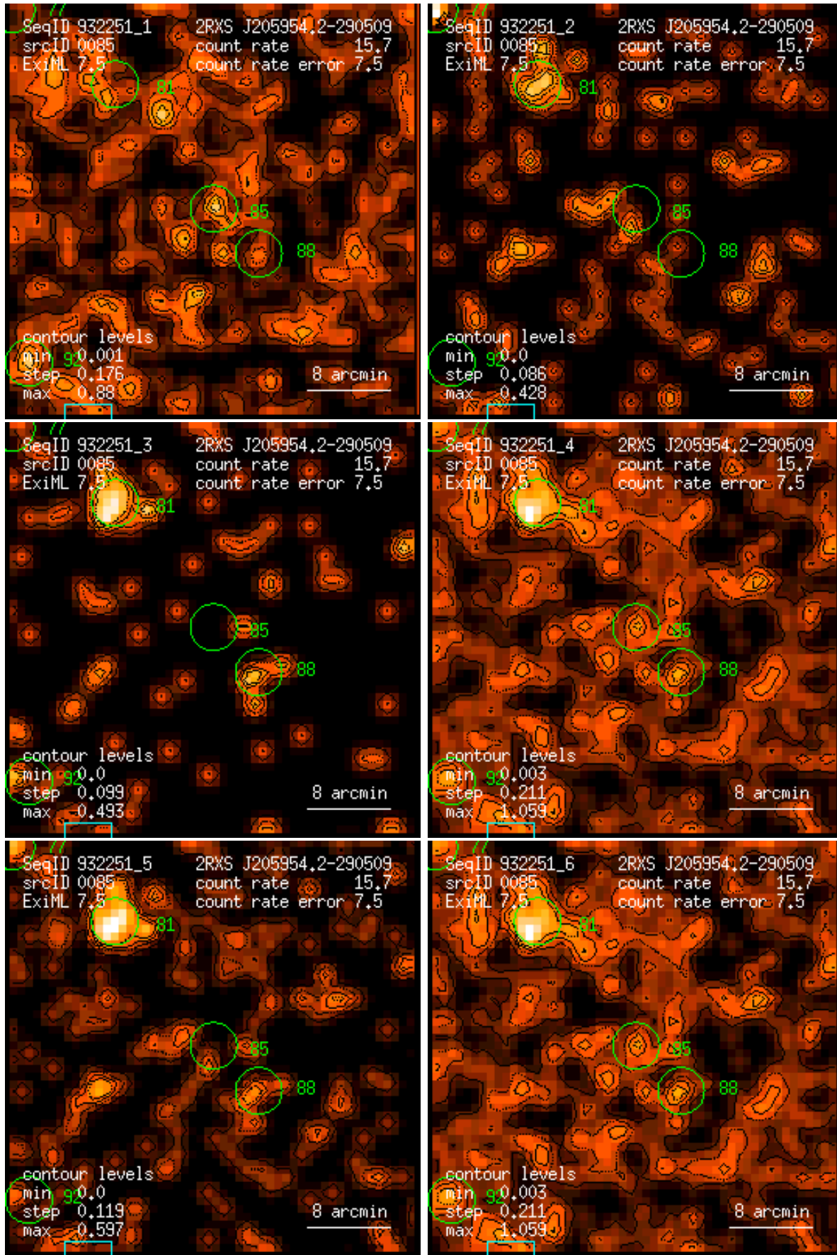
Figure 85: RASS 932251: detection 0085: band rate images, Gaussian filter: (1) PSPC channels 11 – 41, (2) 52 – 90, (3) 91 – 201, (4) 11 – 235, (5) 52 – 201, (6) 11 – 201. Broad band rates in counts/ks. Band rate contour levels in counts/ks/arcmin 2 .
