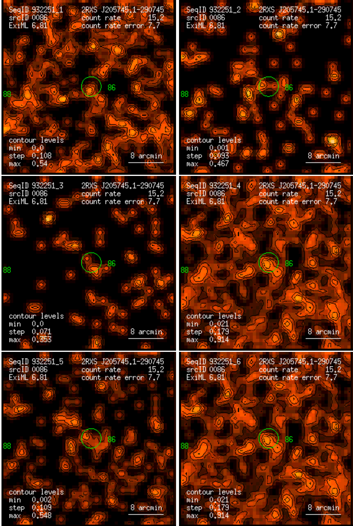
Figure 86: RASS 932251: detection 0086: band rate images, Gaussian filter: (1) PSPC channels 11 – 41, (2) 52 – 90, (3) 91 – 201, (4) 11 – 235, (5) 52 – 201, (6) 11 – 201. Broad band rates in counts/ks. Band rate contour levels in counts/ks/arcmin 2 .
