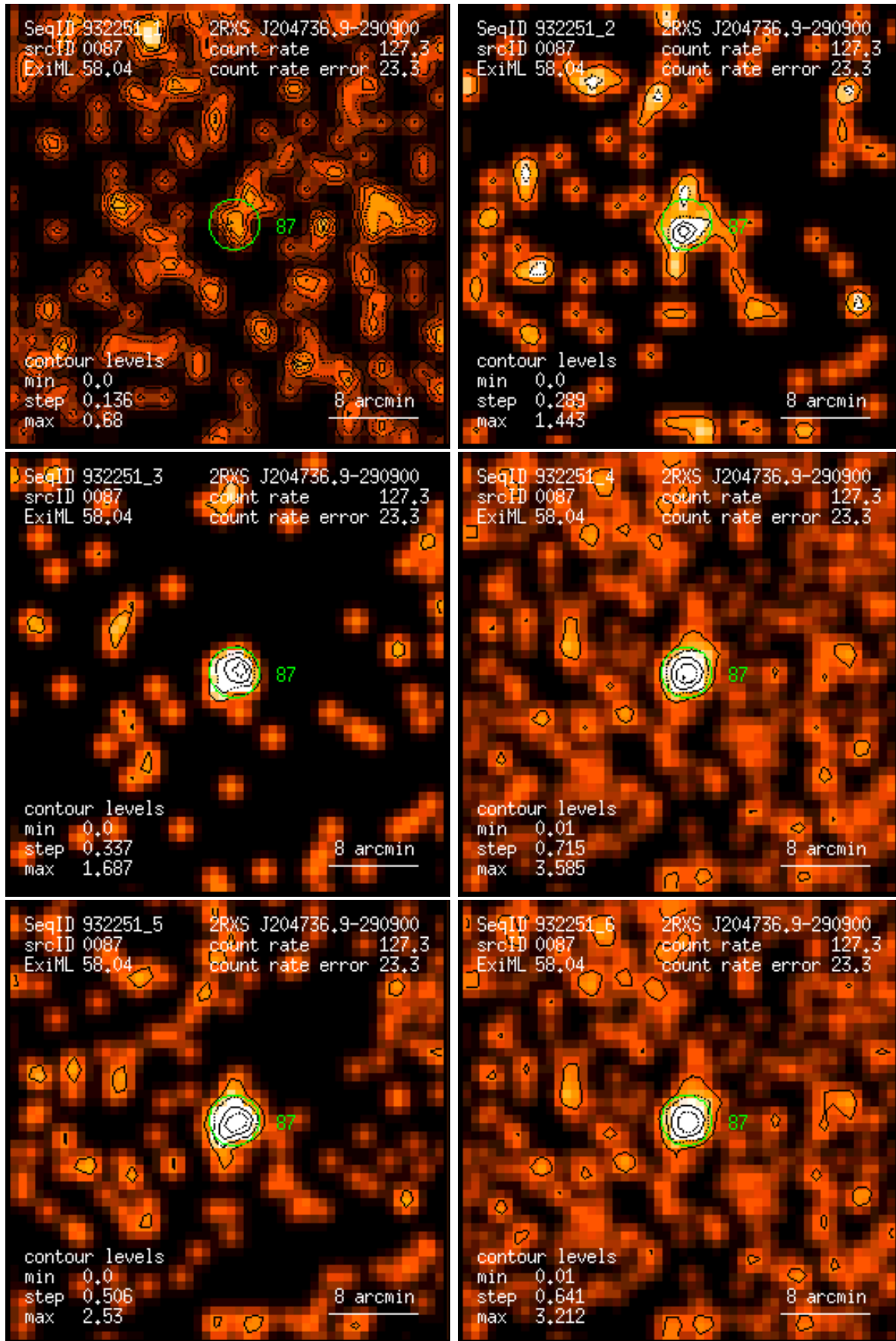
Figure 87: RASS 932251: detection 0087: band rate images, Gaussian filter: (1) PSPC channels 11 – 41, (2) 52 – 90, (3) 91 – 201, (4) 11 – 235, (5) 52 – 201, (6) 11 – 201. Broad band rates in counts/ks. Band rate contour levels in counts/ks/arcmin 2 .
