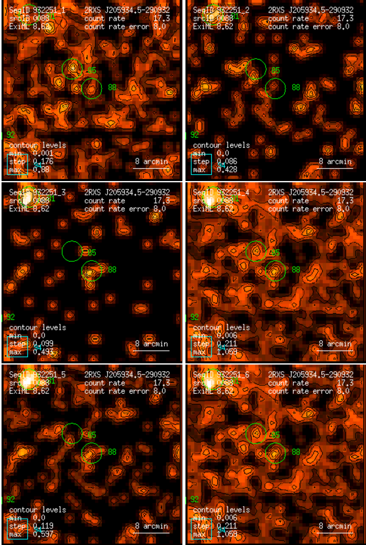
Figure 88: RASS 932251: detection 0088: band rate images, Gaussian filter: (1) PSPC channels 11 – 41, (2) 52 – 90, (3) 91 – 201, (4) 11 – 235, (5) 52 – 201, (6) 11 – 201. Broad band rates in counts/ks. Band rate contour levels in counts/ks/arcmin 2 .
