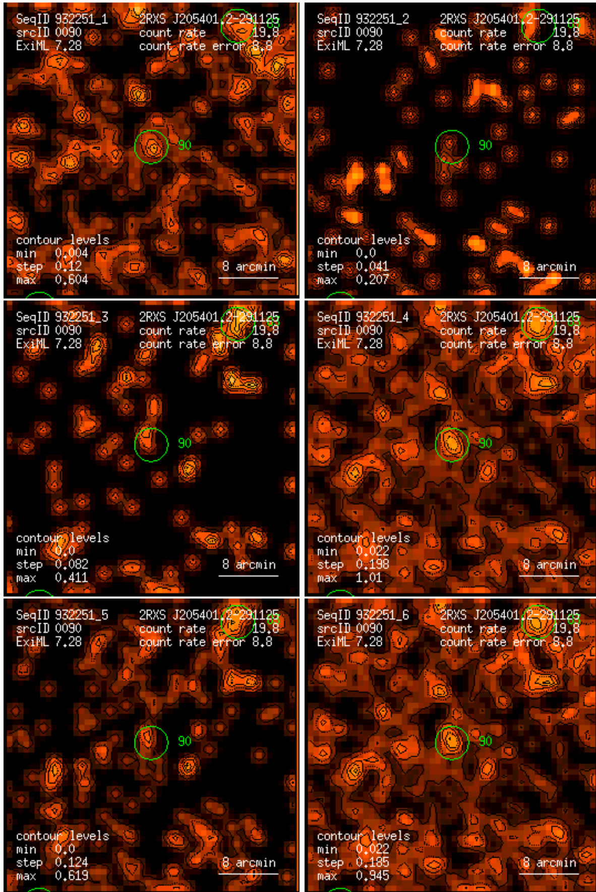
Figure 90: RASS 932251: detection 0090: band rate images, Gaussian filter: (1) PSPC channels 11 – 41, (2) 52 – 90, (3) 91 – 201, (4) 11 – 235, (5) 52 – 201, (6) 11 – 201. Broad band rates in counts/ks. Band rate contour levels in counts/ks/arcmin 2 .
