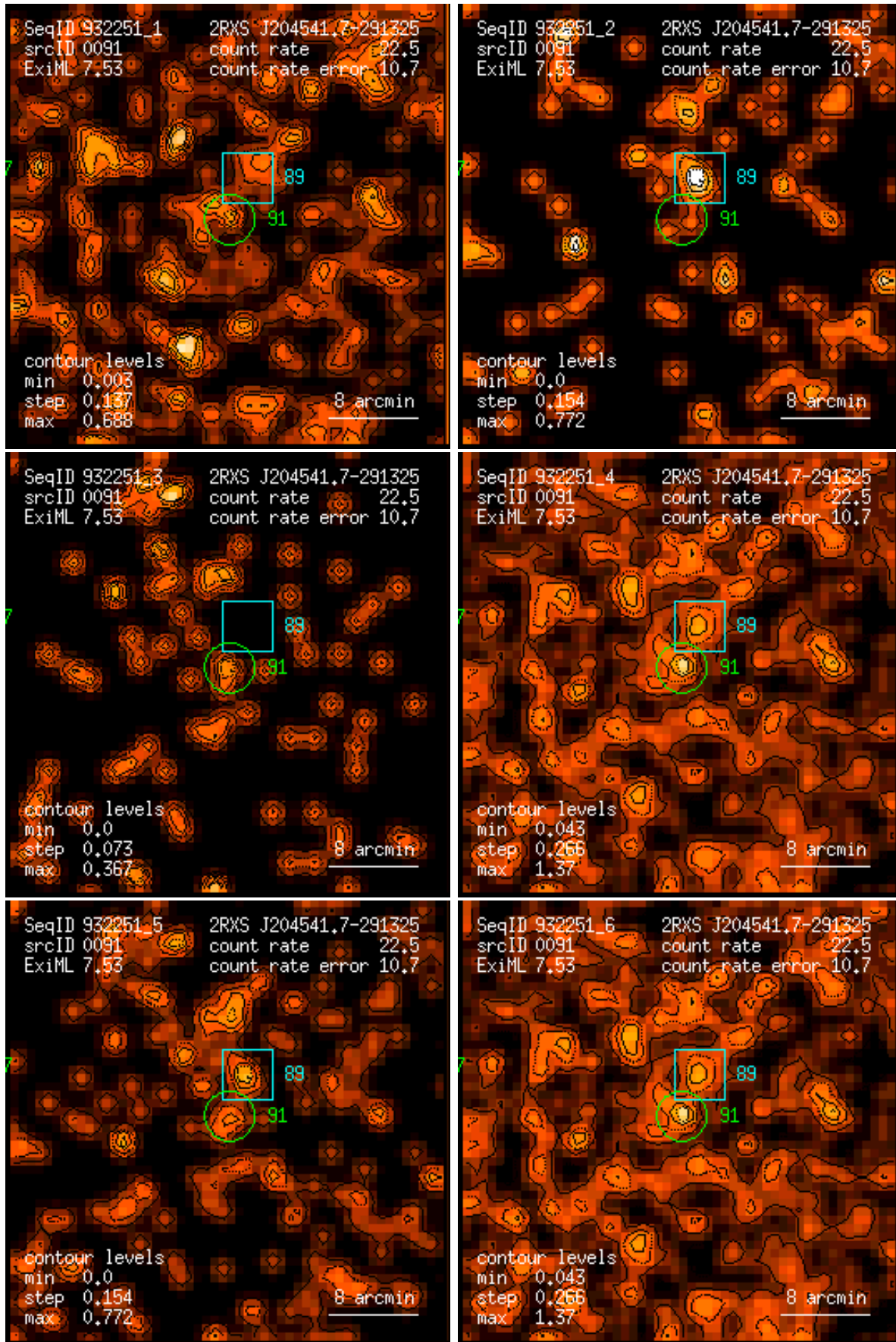
Figure 91: RASS 932251: detection 0091: band rate images, Gaussian filter: (1) PSPC channels 11 – 41, (2) 52 – 90, (3) 91 – 201, (4) 11 – 235, (5) 52 – 201, (6) 11 – 201. Broad band rates in counts/ks. Band rate contour levels in counts/ks/arcmin 2 .
