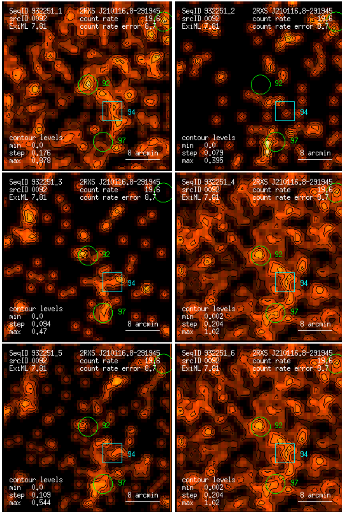
Figure 92: RASS 932251: detection 0092: band rate images, Gaussian filter: (1) PSPC channels 11 – 41, (2) 52 – 90, (3) 91 – 201, (4) 11 – 235, (5) 52 – 201, (6) 11 – 201. Broad band rates in counts/ks. Band rate contour levels in counts/ks/arcmin 2 .
