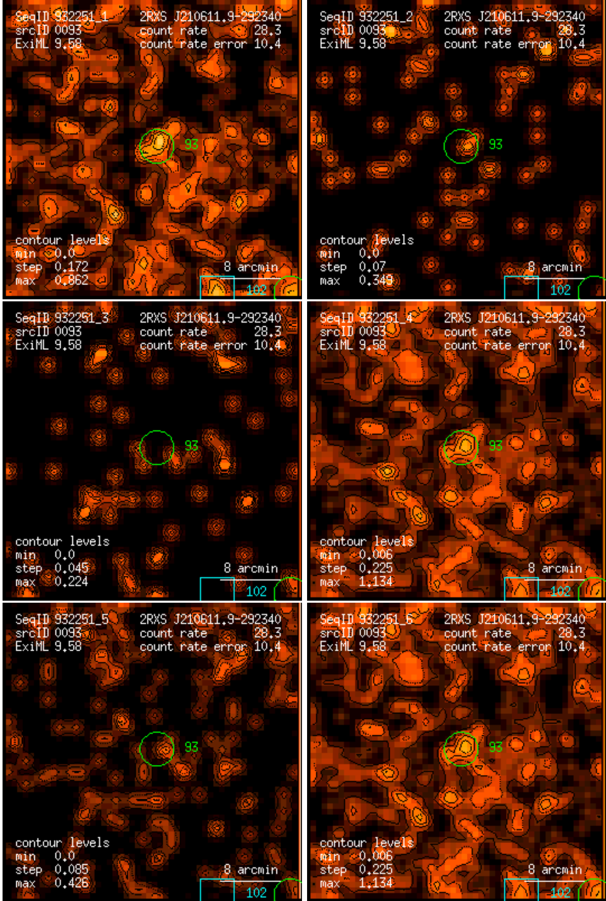
Figure 93: RASS 932251: detection 0093: band rate images, Gaussian filter: (1) PSPC channels 11 – 41, (2) 52 – 90, (3) 91 – 201, (4) 11 – 235, (5) 52 – 201, (6) 11 – 201. Broad band rates in counts/ks. Band rate contour levels in counts/ks/arcmin 2 .
