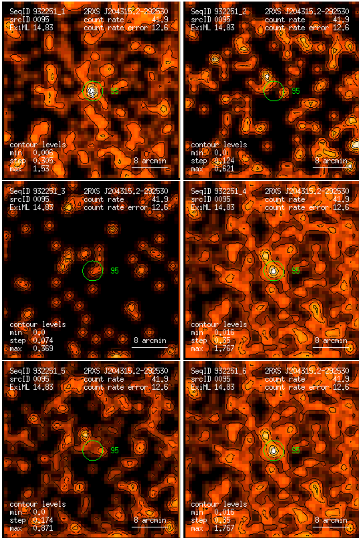
Figure 95: RASS 932251: detection 0095: band rate images, Gaussian filter: (1) PSPC channels 11 – 41, (2) 52 – 90, (3) 91 – 201, (4) 11 – 235, (5) 52 – 201, (6) 11 – 201. Broad band rates in counts/ks. Band rate contour levels in counts/ks/arcmin 2 .
