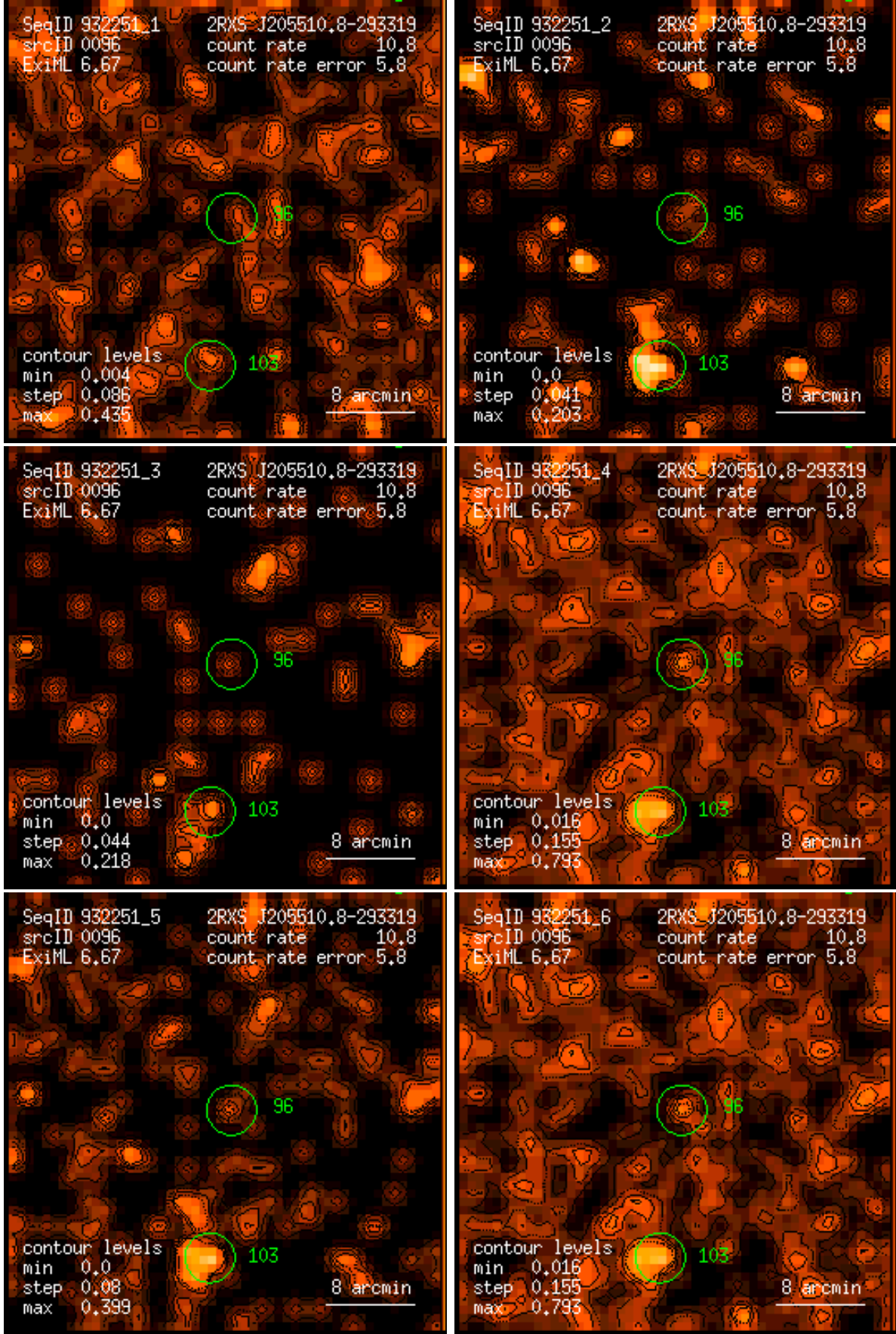
Figure 96: RASS 932251: detection 0096: band rate images, Gaussian filter: (1) PSPC channels 11 – 41, (2) 52 – 90, (3) 91 – 201, (4) 11 – 235, (5) 52 – 201, (6) 11 – 201. Broad band rates in counts/ks. Band rate contour levels in counts/ks/arcmin 2 .
