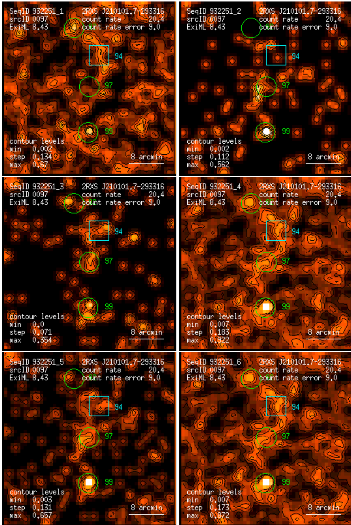
Figure 97: RASS 932251: detection 0097: band rate images, Gaussian filter: (1) PSPC channels 11 – 41, (2) 52 – 90, (3) 91 – 201, (4) 11 – 235, (5) 52 – 201, (6) 11 – 201. Broad band rates in counts/ks. Band rate contour levels in counts/ks/arcmin 2 .
