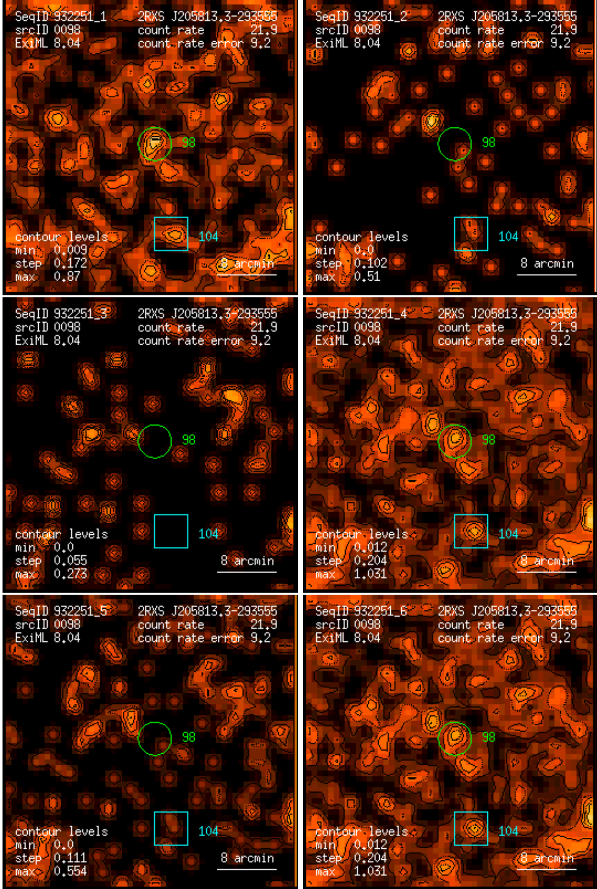
Figure 98: RASS 932251: detection 0098: band rate images, Gaussian filter: (1) PSPC channels 11 – 41, (2) 52 – 90, (3) 91 – 201, (4) 11 – 235, (5) 52 – 201, (6) 11 – 201. Broad band rates in counts/ks. Band rate contour levels in counts/ks/arcmin 2 .
