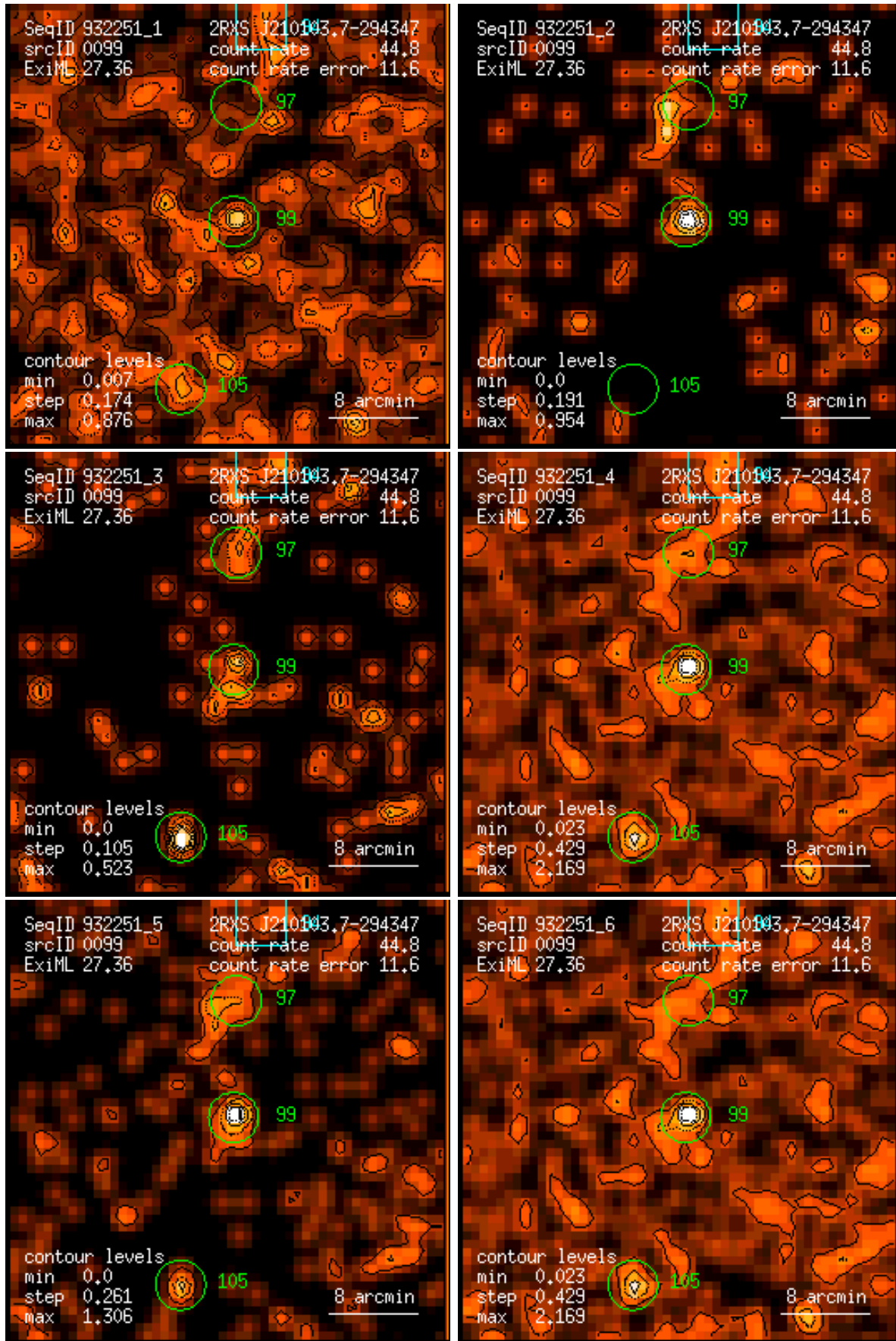
Figure 99: RASS 932251: detection 0099: band rate images, Gaussian filter: (1) PSPC channels 11 – 41, (2) 52 – 90, (3) 91 – 201, (4) 11 – 235, (5) 52 – 201, (6) 11 – 201. Broad band rates in counts/ks. Band rate contour levels in counts/ks/arcmin 2 .
