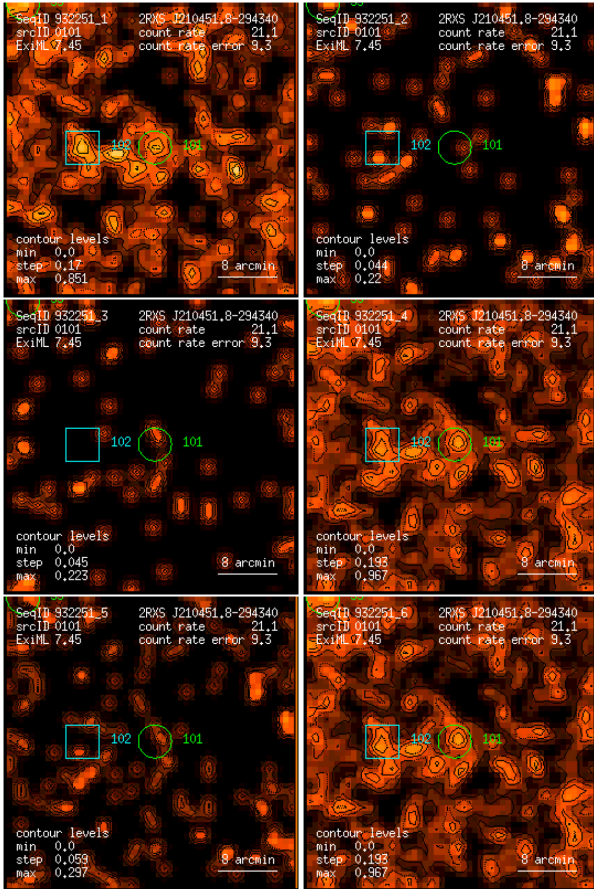
Figure 101: RASS 932251: detection 0101: band rate images, Gaussian filter: (1) PSPC channels 11 – 41, (2) 52 – 90, (3) 91 – 201, (4) 11 – 235, (5) 52 – 201, (6) 11 – 201. Broad band rates in counts/ks. Band rate contour levels in counts/ks/arcmin 2 .
