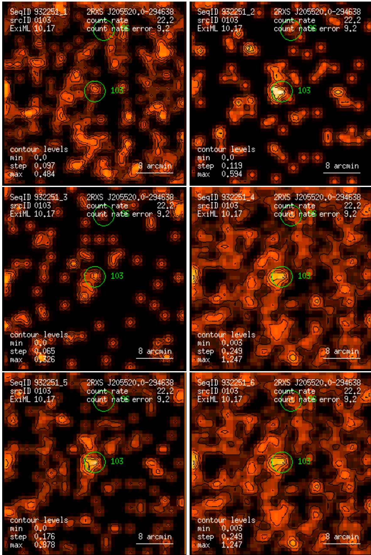
Figure 103: RASS 932251: detection 0103: band rate images, Gaussian filter: (1) PSPC channels 11 – 41, (2) 52 – 90, (3) 91 – 201, (4) 11 – 235, (5) 52 – 201, (6) 11 – 201. Broad band rates in counts/ks. Band rate contour levels in counts/ks/arcmin 2 .
