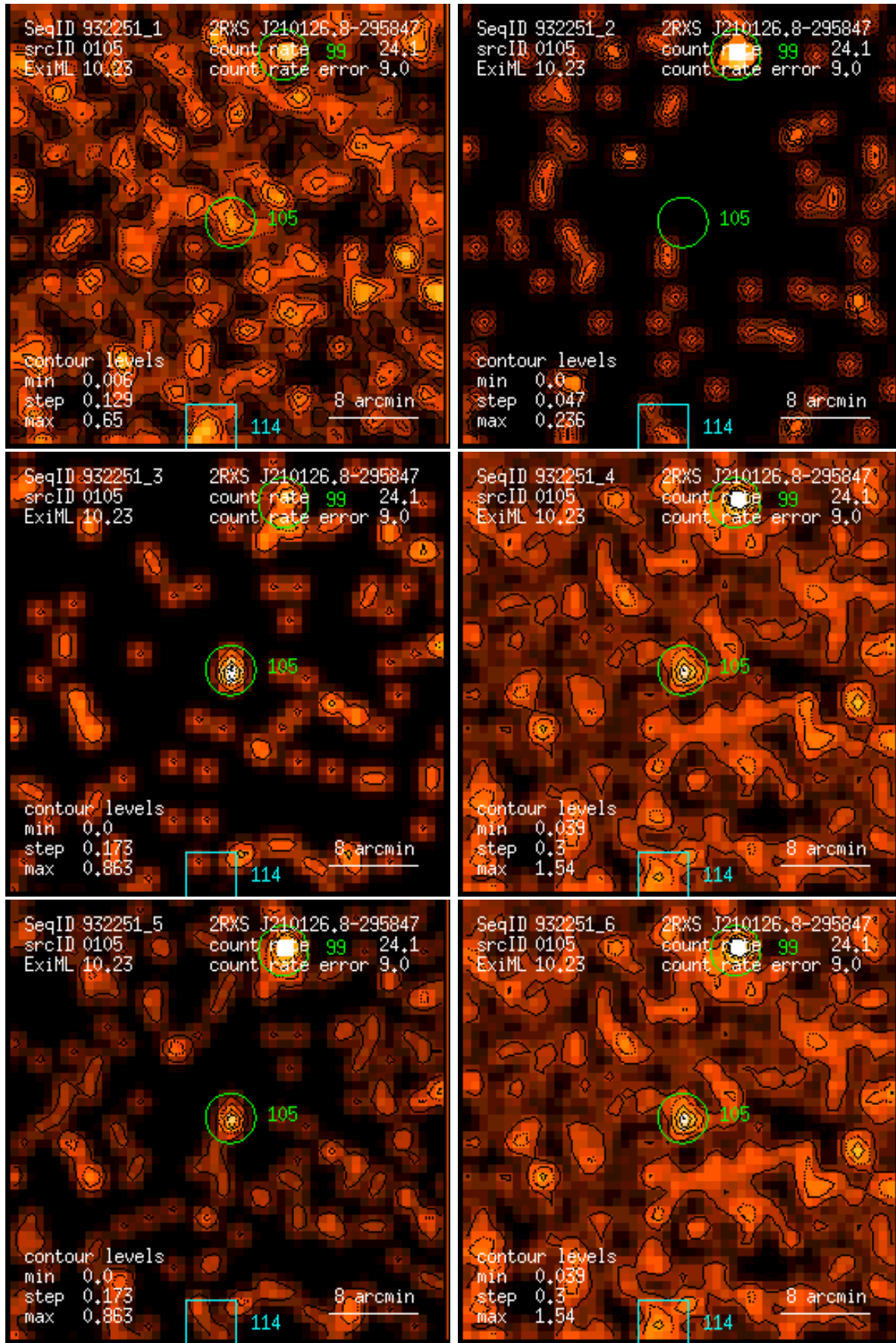
Figure 105: RASS 932251: detection 0105: band rate images, Gaussian filter: (1) PSPC channels 11 – 41, (2) 52 – 90, (3) 91 – 201, (4) 11 – 235, (5) 52 – 201, (6) 11 – 201. Broad band rates in counts/ks. Band rate contour levels in counts/ks/arcmin 2 .
