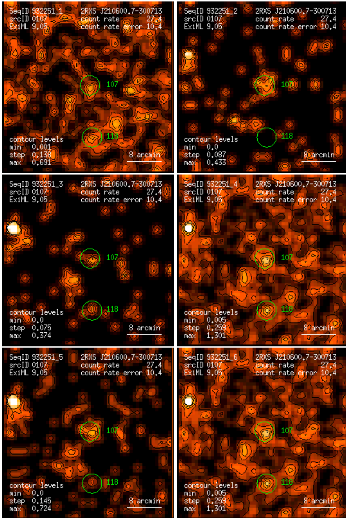
Figure 107: RASS 932251: detection 0107: band rate images, Gaussian filter: (1) PSPC channels 11 – 41, (2) 52 – 90, (3) 91 – 201, (4) 11 – 235, (5) 52 – 201, (6) 11 – 201. Broad band rates in counts/ks. Band rate contour levels in counts/ks/arcmin 2 .
