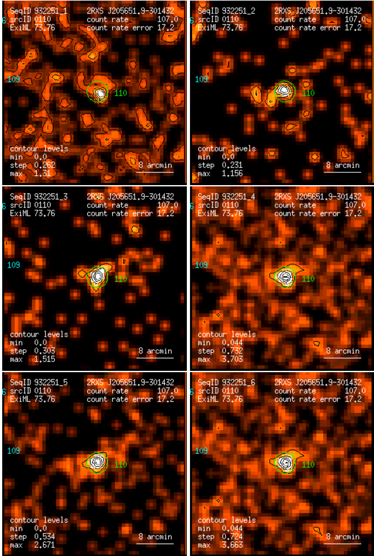
Figure 110: RASS 932251: detection 0110: band rate images, Gaussian filter: (1) PSPC channels 11 – 41, (2) 52 – 90, (3) 91 – 201, (4) 11 – 235, (5) 52 – 201, (6) 11 – 201. Broad band rates in counts/ks. Band rate contour levels in counts/ks/arcmin 2 .
