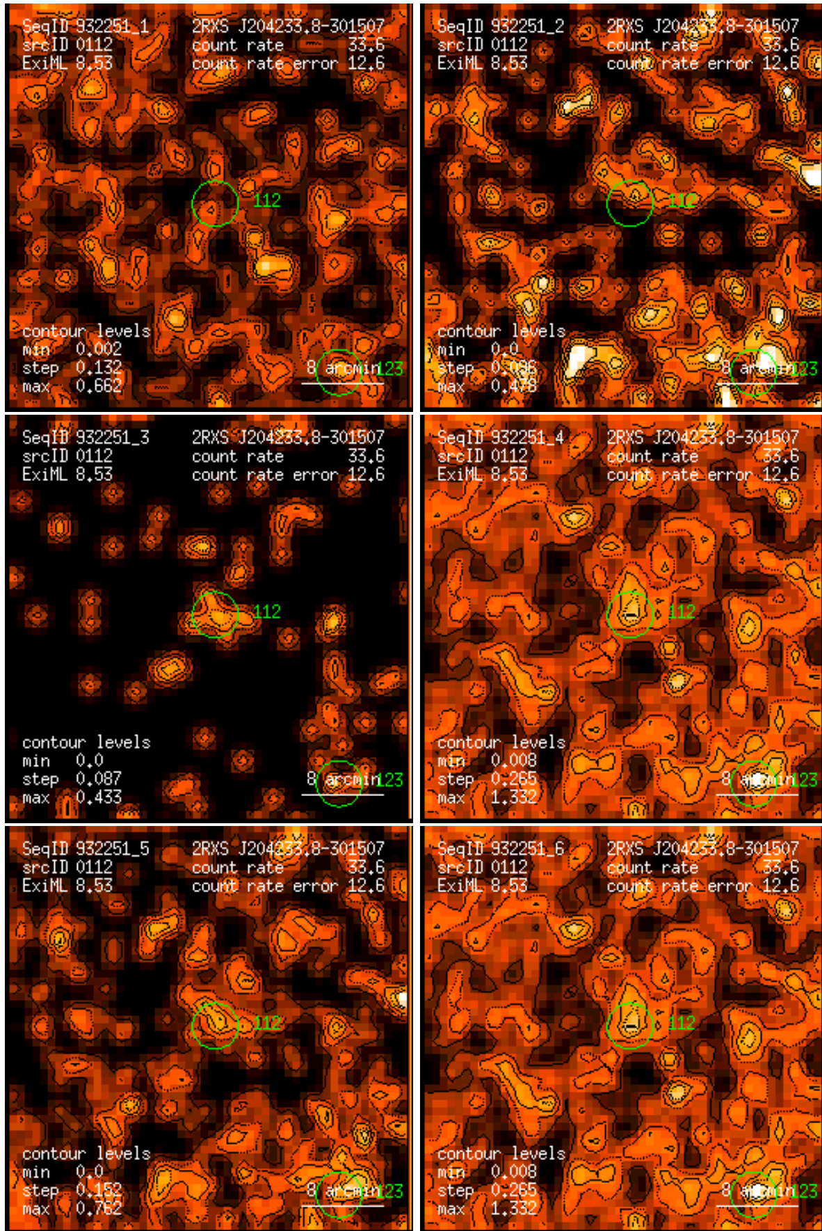
Figure 112: RASS 932251: detection 0112: band rate images, Gaussian filter: (1) PSPC channels 11 – 41, (2) 52 – 90, (3) 91 – 201, (4) 11 – 235, (5) 52 – 201, (6) 11 – 201. Broad band rates in counts/ks. Band rate contour levels in counts/ks/arcmin 2 .
