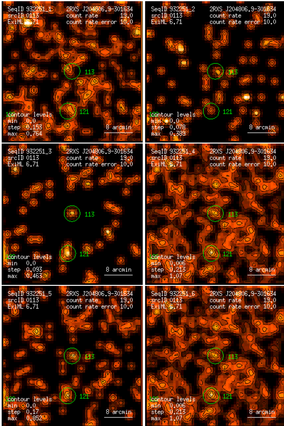
Figure 113: RASS 932251: detection 0113: band rate images, Gaussian filter: (1) PSPC channels 11 – 41, (2) 52 – 90, (3) 91 – 201, (4) 11 – 235, (5) 52 – 201, (6) 11 – 201. Broad band rates in counts/ks. Band rate contour levels in counts/ks/arcmin 2 .
