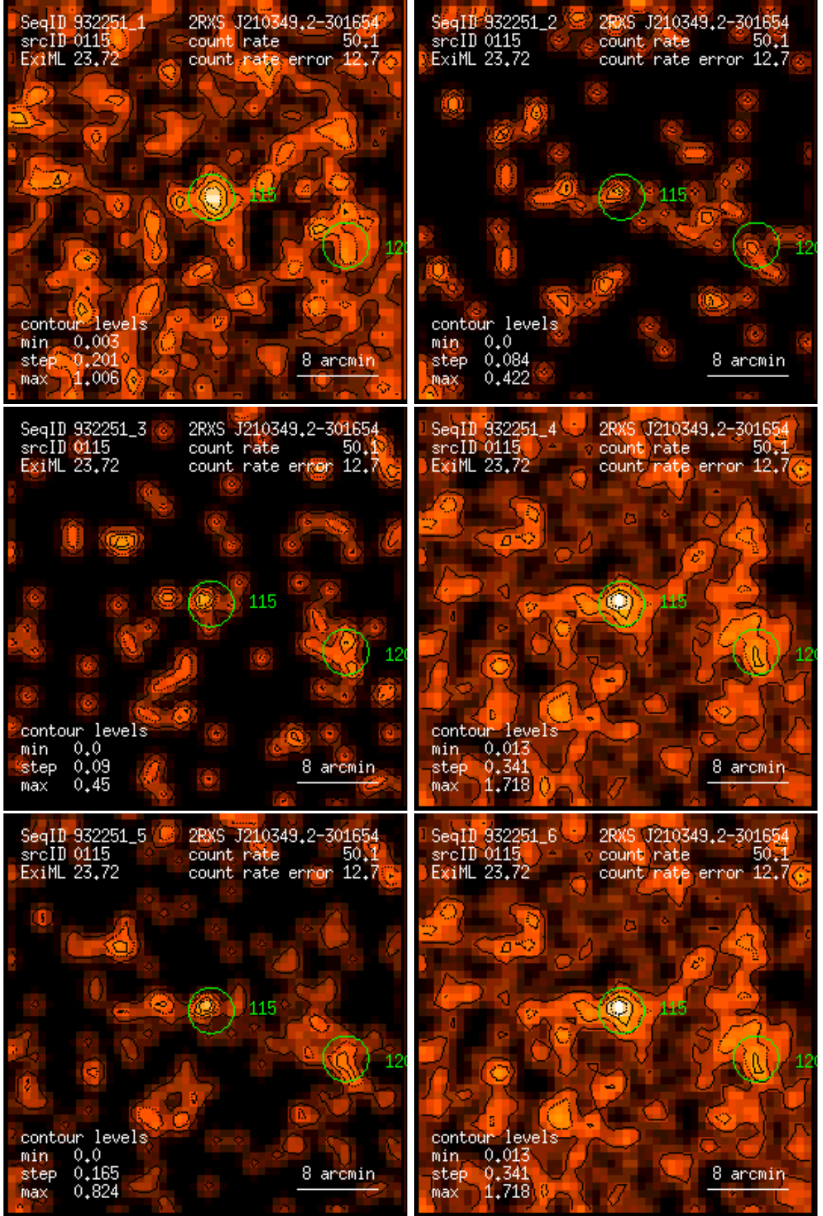
Figure 115: RASS 932251: detection 0115: band rate images, Gaussian filter: (1) PSPC channels 11 – 41, (2) 52 – 90, (3) 91 – 201, (4) 11 – 235, (5) 52 – 201, (6) 11 – 201. Broad band rates in counts/ks. Band rate contour levels in counts/ks/arcmin 2 .
