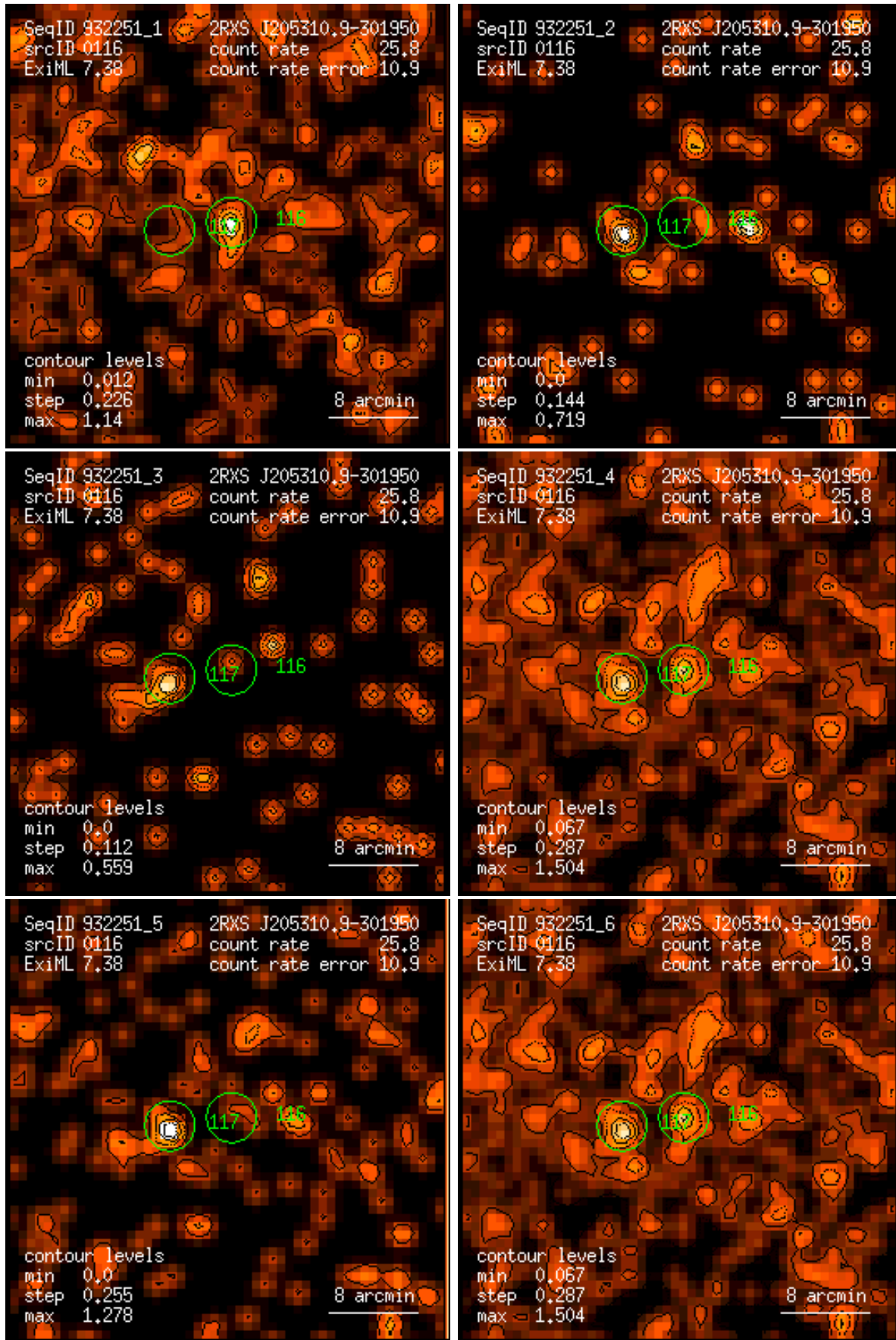
Figure 116: RASS 932251: detection 0116: band rate images, Gaussian filter: (1) PSPC channels 11 – 41, (2) 52 – 90, (3) 91 – 201, (4) 11 – 235, (5) 52 – 201, (6) 11 – 201. Broad band rates in counts/ks. Band rate contour levels in counts/ks/arcmin 2 .
