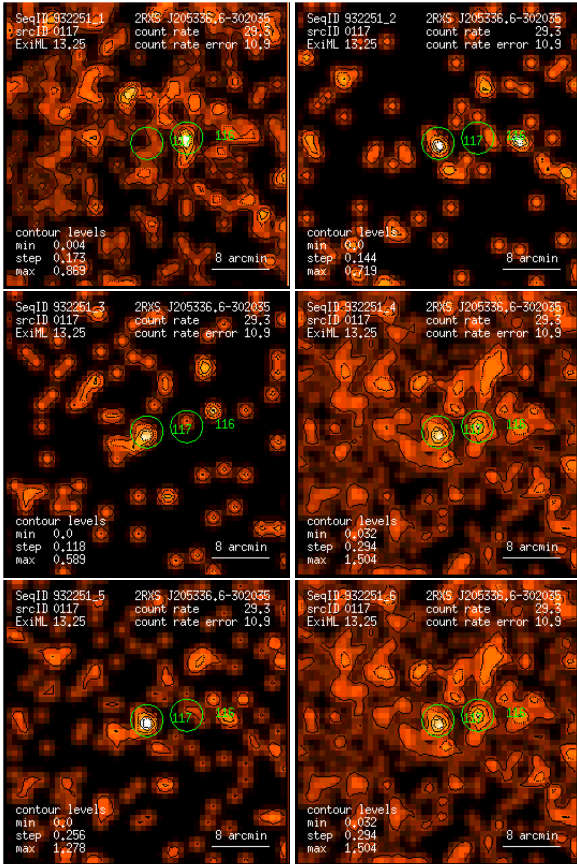
Figure 117: RASS 932251: detection 0117: band rate images, Gaussian filter: (1) PSPC channels 11 – 41, (2) 52 – 90, (3) 91 – 201, (4) 11 – 235, (5) 52 – 201, (6) 11 – 201. Broad band rates in counts/ks. Band rate contour levels in counts/ks/arcmin 2 .
