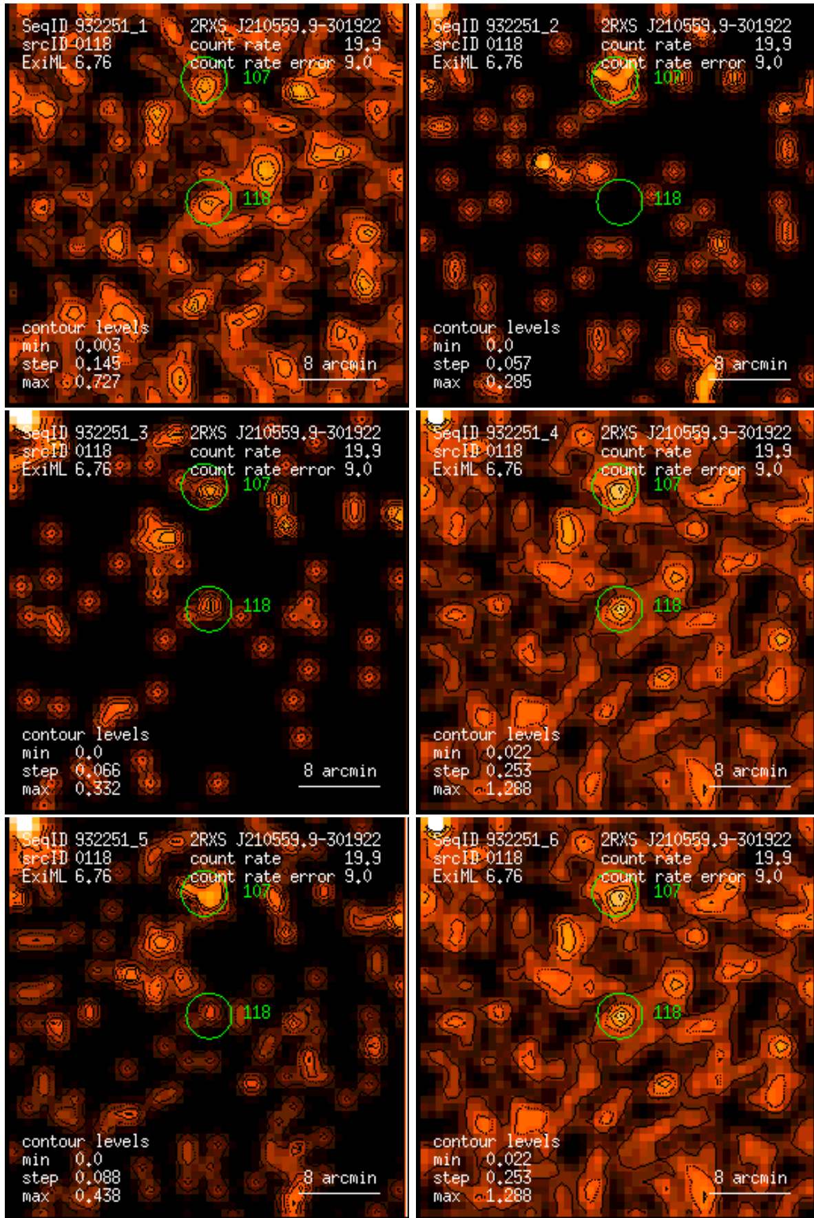
Figure 118: RASS 932251: detection 0118: band rate images, Gaussian filter: (1) PSPC channels 11 – 41, (2) 52 – 90, (3) 91 – 201, (4) 11 – 235, (5) 52 – 201, (6) 11 – 201. Broad band rates in counts/ks. Band rate contour levels in counts/ks/arcmin 2 .
