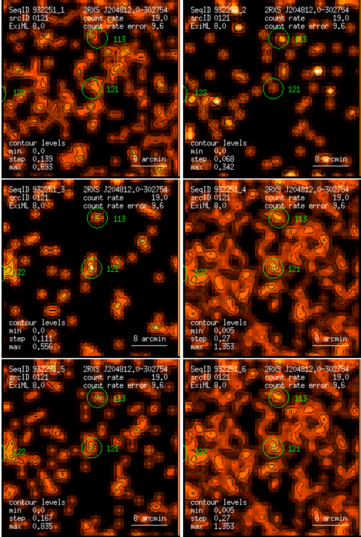
Figure 121: RASS 932251: detection 0121: band rate images, Gaussian filter: (1) PSPC channels 11 – 41, (2) 52 – 90, (3) 91 – 201, (4) 11 – 235, (5) 52 – 201, (6) 11 – 201. Broad band rates in counts/ks. Band rate contour levels in counts/ks/arcmin 2 .
