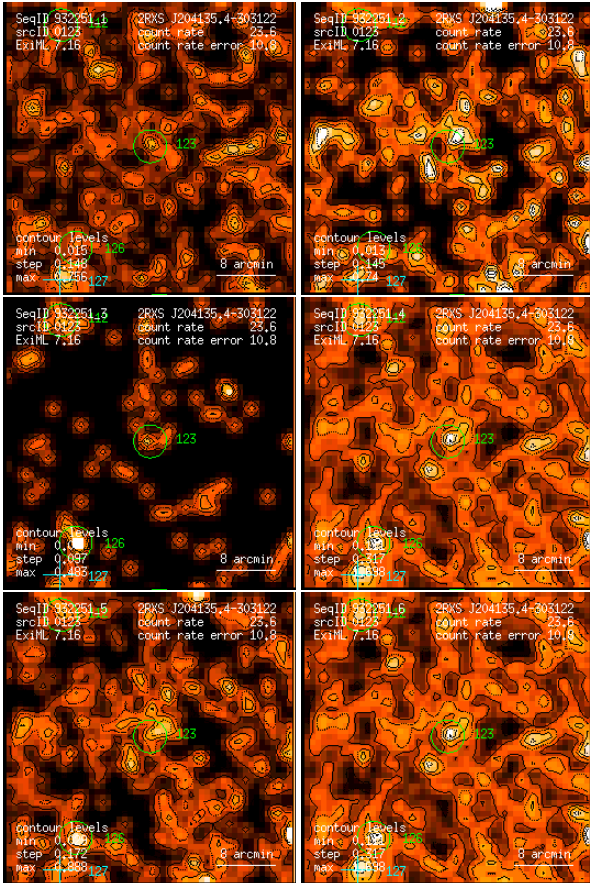
Figure 123: RASS 932251: detection 0123: band rate images, Gaussian filter: (1) PSPC channels 11 – 41, (2) 52 – 90, (3) 91 – 201, (4) 11 – 235, (5) 52 – 201, (6) 11 – 201. Broad band rates in counts/ks. Band rate contour levels in counts/ks/arcmin 2 .
