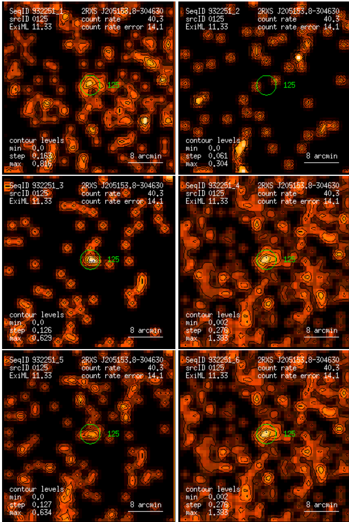
Figure 125: RASS 932251: detection 0125: band rate images, Gaussian filter: (1) PSPC channels 11 – 41, (2) 52 – 90, (3) 91 – 201, (4) 11 – 235, (5) 52 – 201, (6) 11 – 201. Broad band rates in counts/ks. Band rate contour levels in counts/ks/arcmin 2 .
