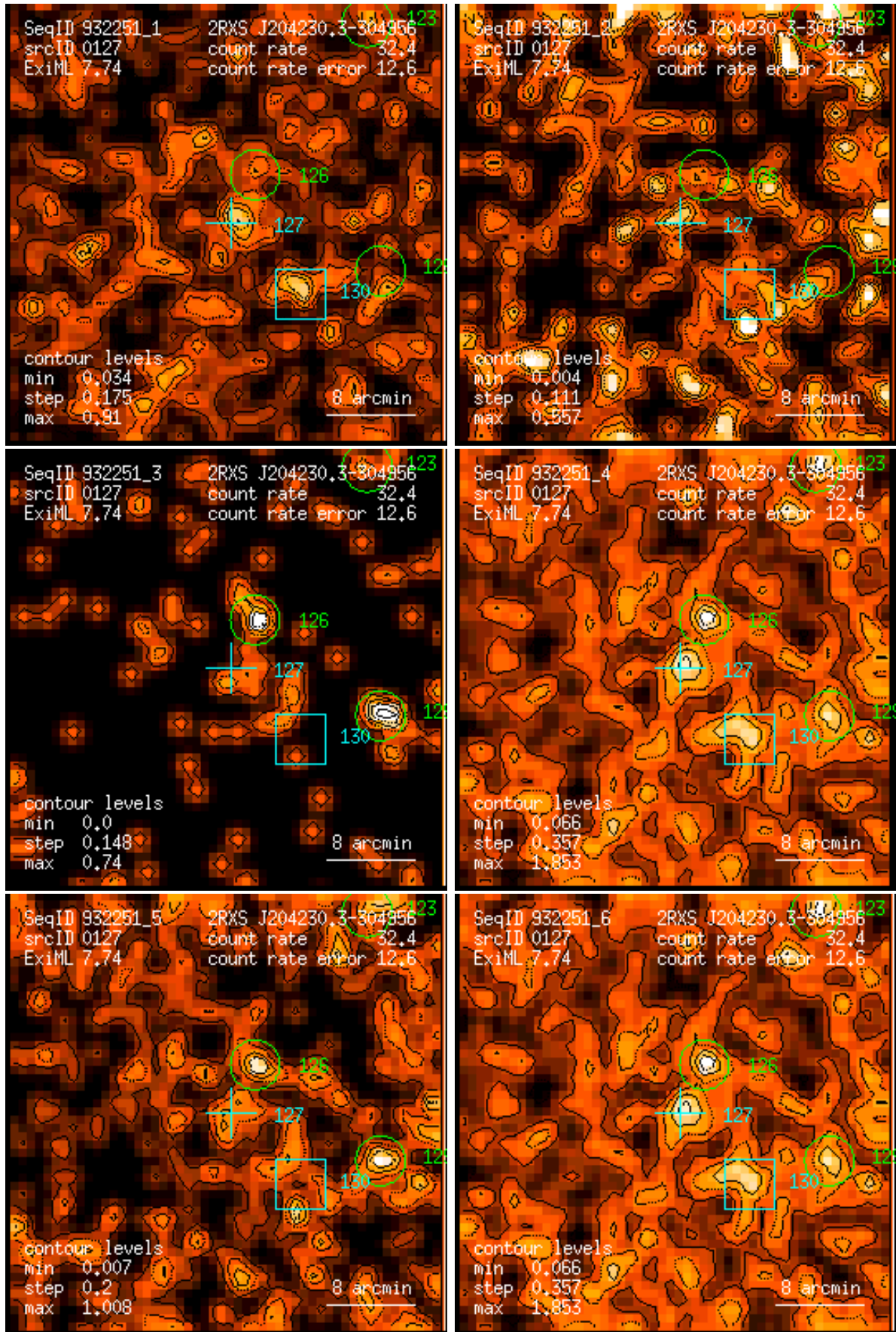
Figure 127: RASS 932251: detection 0127: band rate images, Gaussian filter: (1) PSPC channels 11 – 41, (2) 52 – 90, (3) 91 – 201, (4) 11 – 235, (5) 52 – 201, (6) 11 – 201. Broad band rates in counts/ks. Band rate contour levels in counts/ks/arcmin 2 .
