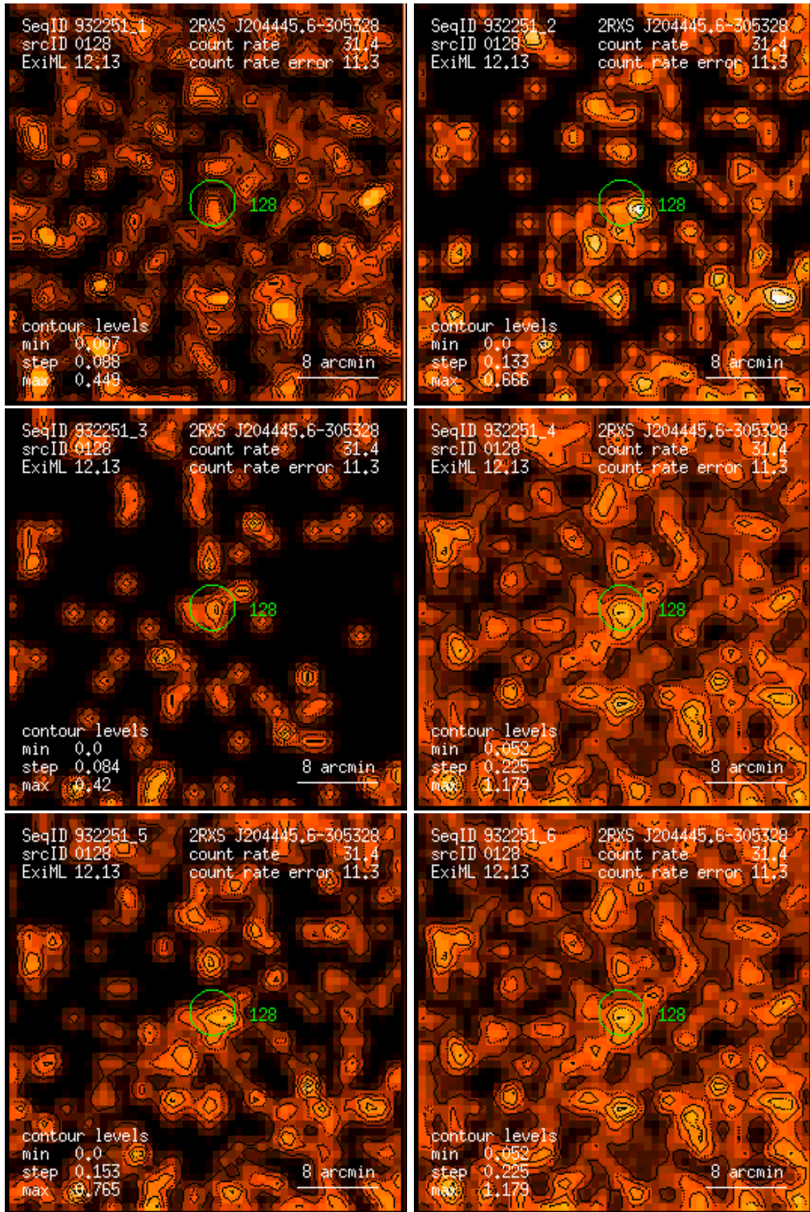
Figure 128: RASS 932251: detection 0128: band rate images, Gaussian filter: (1) PSPC channels 11 – 41, (2) 52 – 90, (3) 91 – 201, (4) 11 – 235, (5) 52 – 201, (6) 11 – 201. Broad band rates in counts/ks. Band rate contour levels in counts/ks/arcmin 2 .
