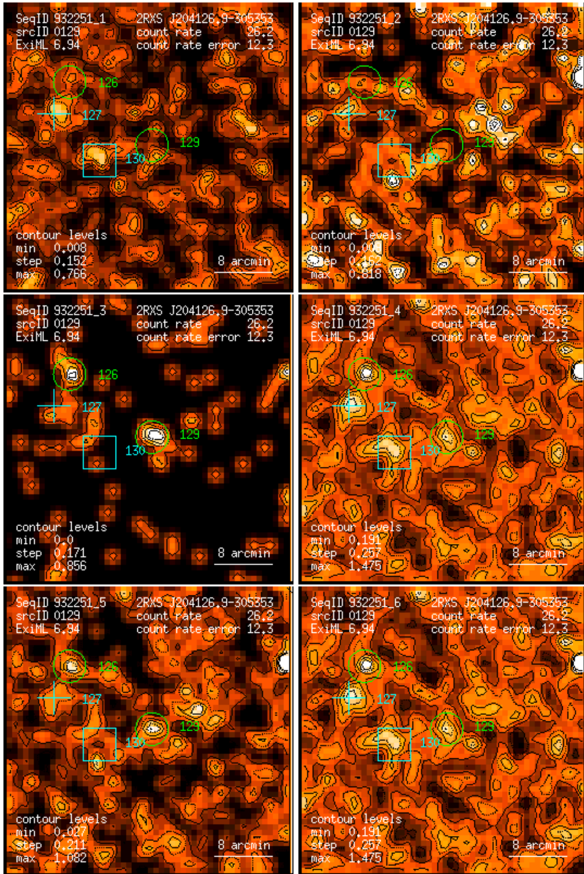
Figure 129: RASS 932251: detection 0129: band rate images, Gaussian filter: (1) PSPC channels 11 – 41, (2) 52 – 90, (3) 91 – 201, (4) 11 – 235, (5) 52 – 201, (6) 11 – 201. Broad band rates in counts/ks. Band rate contour levels in counts/ks/arcmin 2 .
