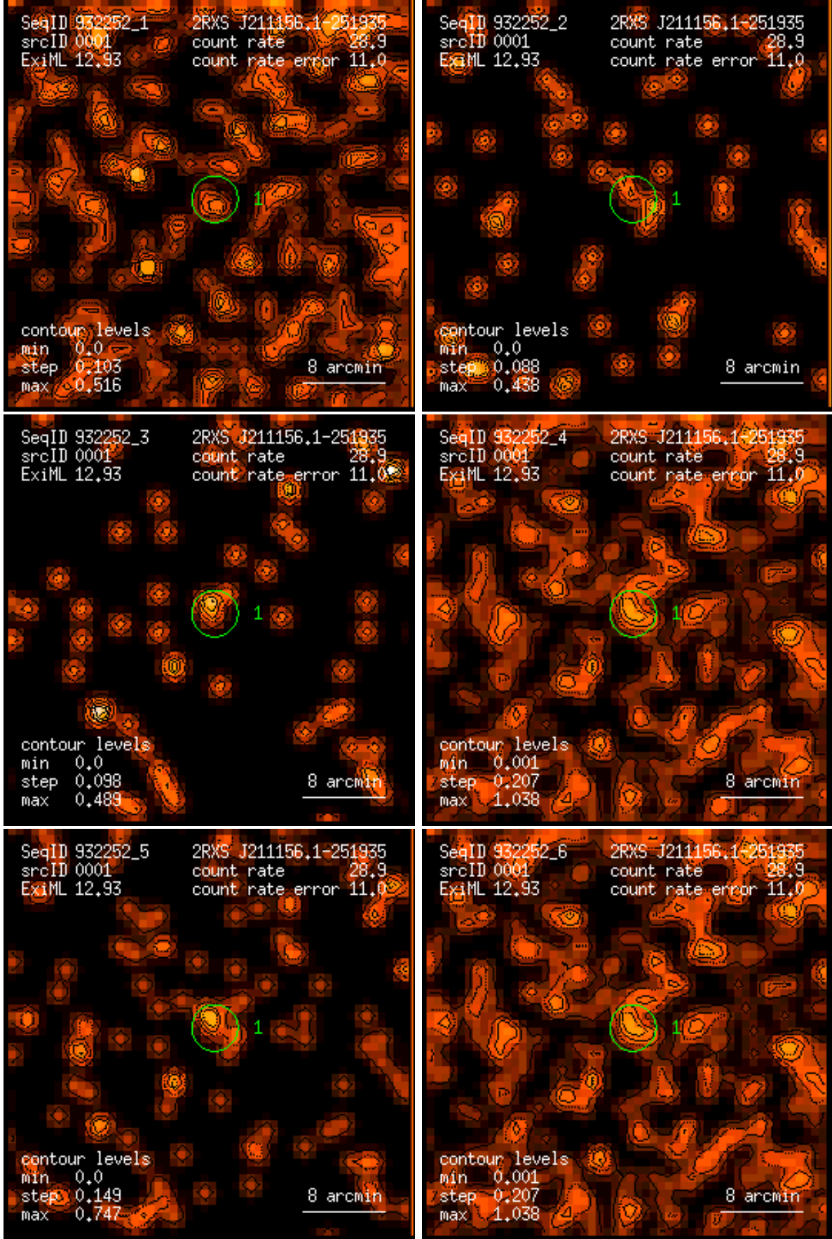
Figure 1: RASS 932252: detection 0001: band rate images, Gaussian filter: (1) PSPC channels 11 – 41, (2) 52 – 90, (3) 91 – 201, (4) 11 – 235, (5) 52 – 201, (6) 11 – 201. Broad band rates in counts/ks. Band rate contour levels in counts/ks/arcmin 2 .
