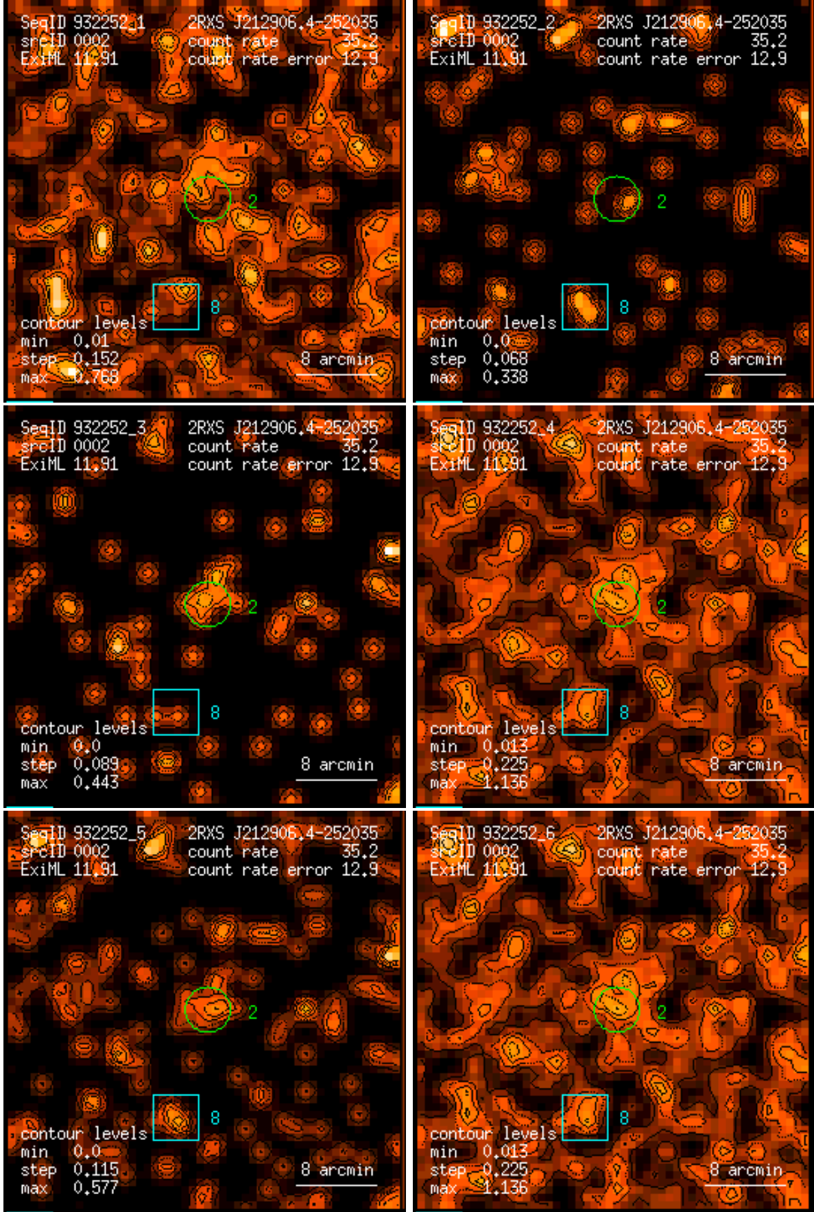
Figure 2: RASS 932252: detection 0002: band rate images, Gaussian filter: (1) PSPC channels 11 – 41, (2) 52 – 90, (3) 91 – 201, (4) 11 – 235, (5) 52 – 201, (6) 11 – 201. Broad band rates in counts/ks. Band rate contour levels in counts/ks/arcmin 2 .
