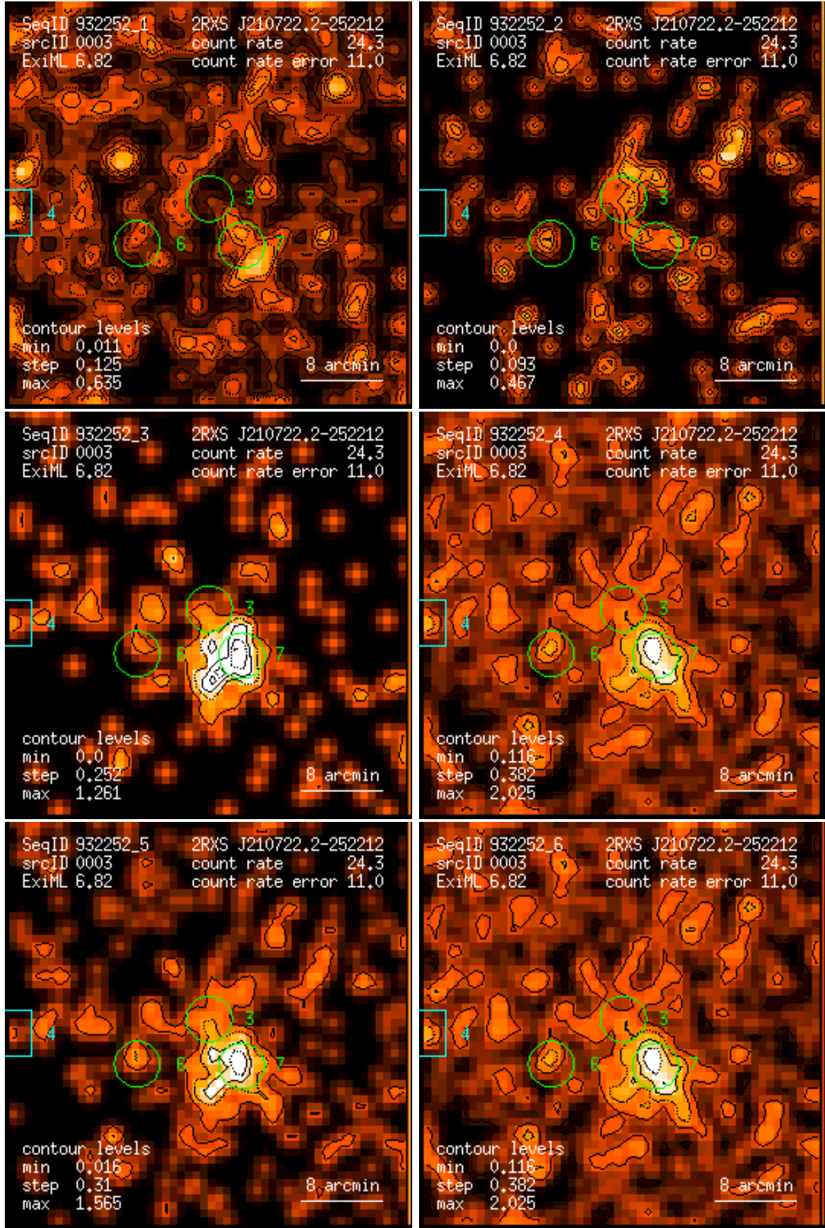
Figure 3: RASS 932252: detection 0003: band rate images, Gaussian filter: (1) PSPC channels 11 – 41, (2) 52 – 90, (3) 91 – 201, (4) 11 – 235, (5) 52 – 201, (6) 11 – 201. Broad band rates in counts/ks. Band rate contour levels in counts/ks/arcmin 2 .
