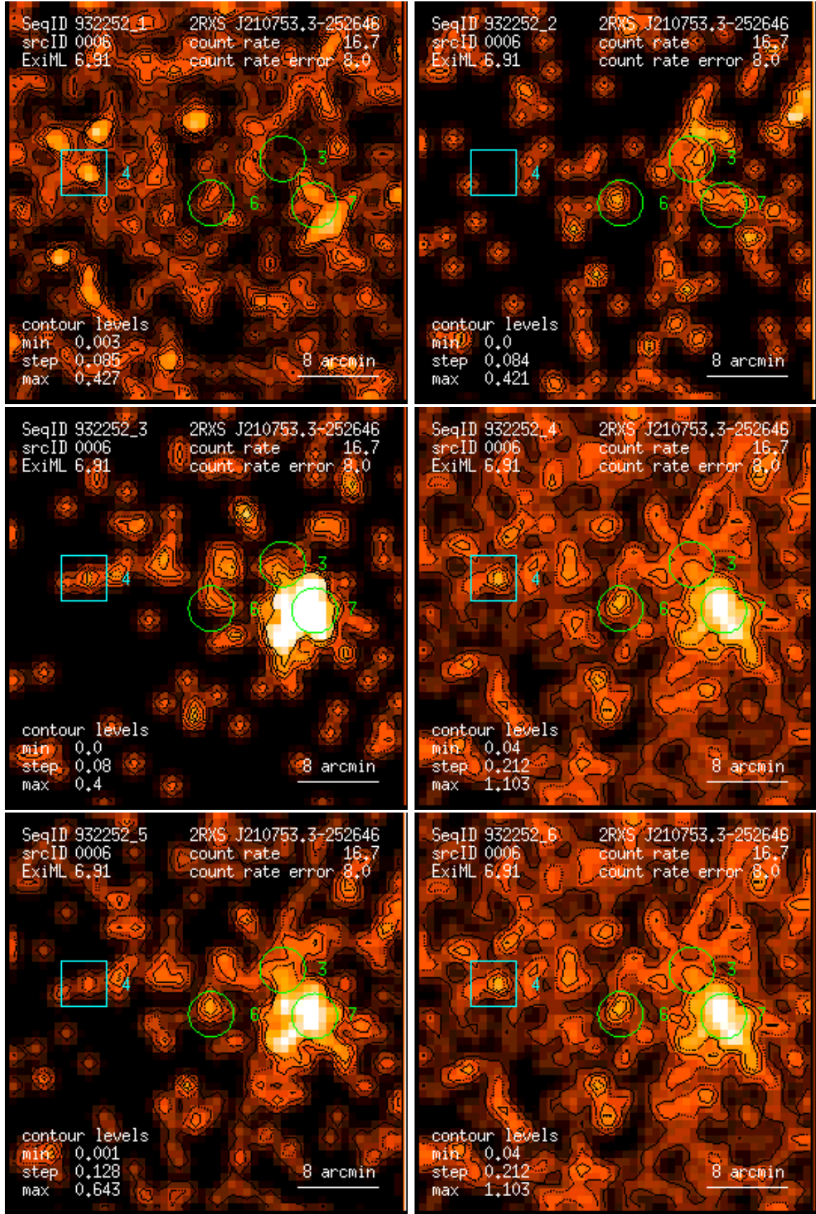
Figure 6: RASS 932252: detection 0006: band rate images, Gaussian filter: (1) PSPC channels 11 – 41, (2) 52 – 90, (3) 91 – 201, (4) 11 – 235, (5) 52 – 201, (6) 11 – 201. Broad band rates in counts/ks. Band rate contour levels in counts/ks/arcmin 2 .
