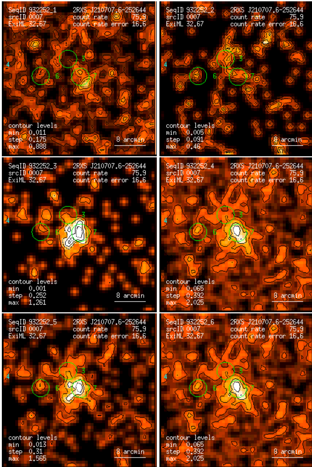
Figure 7: RASS 932252: detection 0007: band rate images, Gaussian filter: (1) PSPC channels 11 – 41, (2) 52 – 90, (3) 91 – 201, (4) 11 – 235, (5) 52 – 201, (6) 11 – 201. Broad band rates in counts/ks. Band rate contour levels in counts/ks/arcmin 2 .
