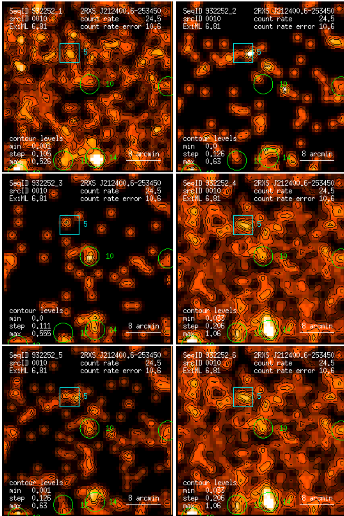
Figure 10: RASS 932252: detection 0010: band rate images, Gaussian filter: (1) PSPC channels 11 – 41, (2) 52 – 90, (3) 91 – 201, (4) 11 – 235, (5) 52 – 201, (6) 11 – 201. Broad band rates in counts/ks. Band rate contour levels in counts/ks/arcmin 2 .
