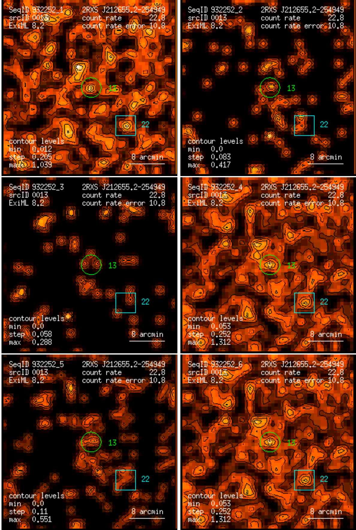
Figure 13: RASS 932252: detection 0013: band rate images, Gaussian filter: (1) PSPC channels 11 – 41, (2) 52 – 90, (3) 91 – 201, (4) 11 – 235, (5) 52 – 201, (6) 11 – 201. Broad band rates in counts/ks. Band rate contour levels in counts/ks/arcmin 2 .
